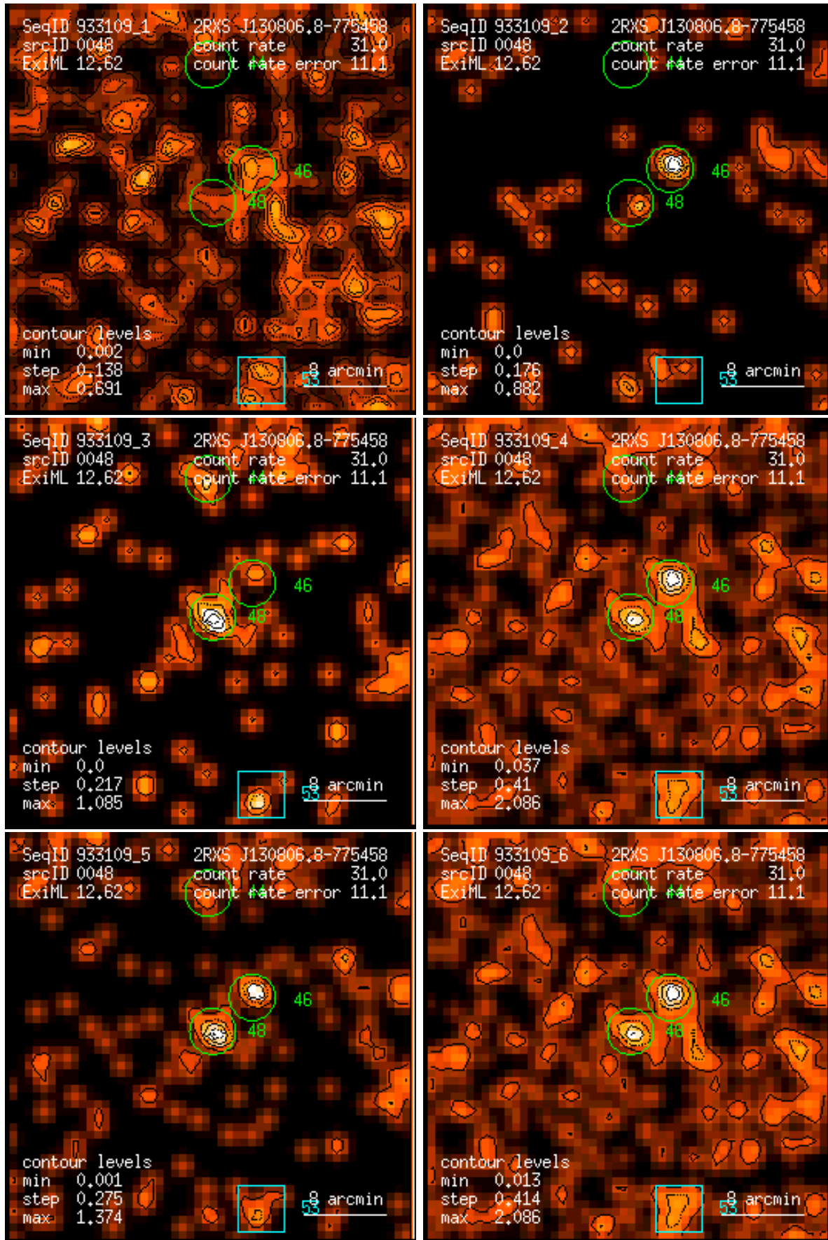
Figure 48: RASS 933109: detection 0048: band rate images, Gaussian filter: (1) PSPC channels 11 – 41, (2) 52 – 90, (3) 91 – 201, (4) 11 – 235, (5) 52 – 201, (6) 11 – 201. Broad band rates in counts/ks. Band rate contour levels in counts/ks/arcmin 2 .
