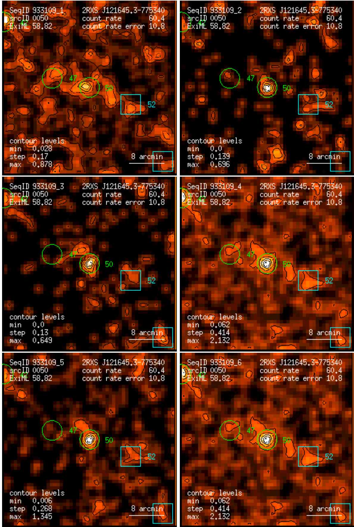
Figure 50: RASS 933109: detection 0050: band rate images, Gaussian filter: (1) PSPC channels 11 – 41, (2) 52 – 90, (3) 91 – 201, (4) 11 – 235, (5) 52 – 201, (6) 11 – 201. Broad band rates in counts/ks. Band rate contour levels in counts/ks/arcmin 2 .
