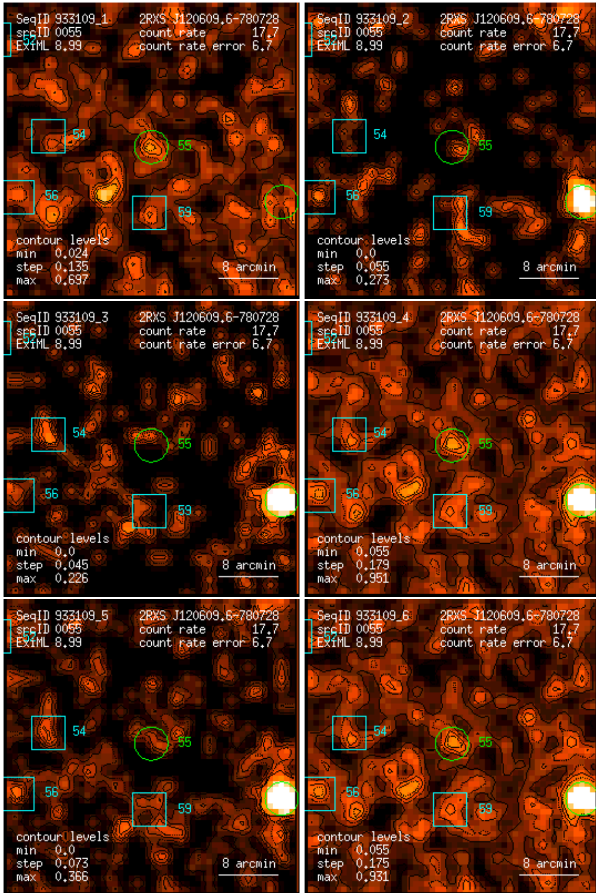
Figure 55: RASS 933109: detection 0055: band rate images, Gaussian filter: (1) PSPC channels 11 – 41, (2) 52 – 90, (3) 91 – 201, (4) 11 – 235, (5) 52 – 201, (6) 11 – 201. Broad band rates in counts/ks. Band rate contour levels in counts/ks/arcmin 2 .
