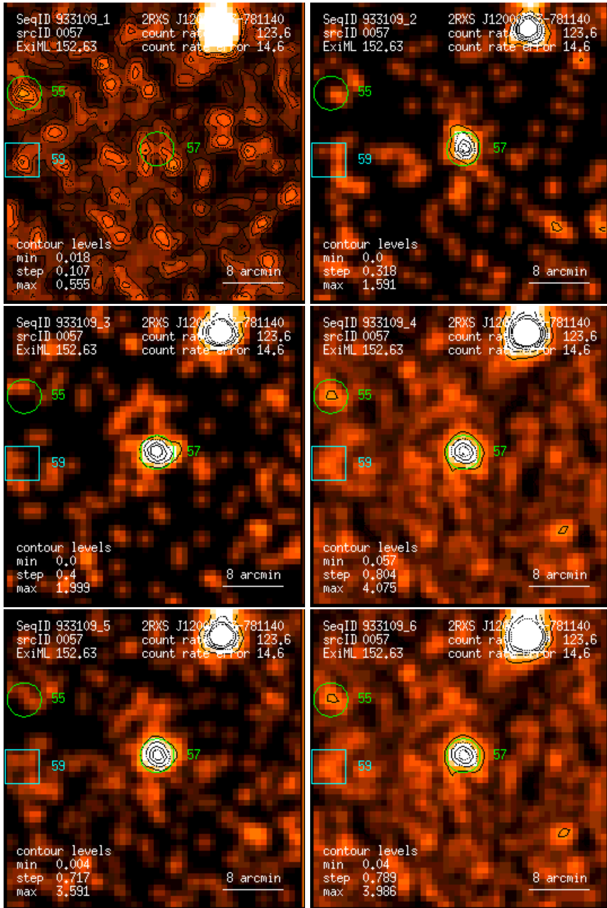
Figure 57: RASS 933109: detection 0057: band rate images, Gaussian filter: (1) PSPC channels 11 – 41, (2) 52 – 90, (3) 91 – 201, (4) 11 – 235, (5) 52 – 201, (6) 11 – 201. Broad band rates in counts/ks. Band rate contour levels in counts/ks/arcmin 2 .
