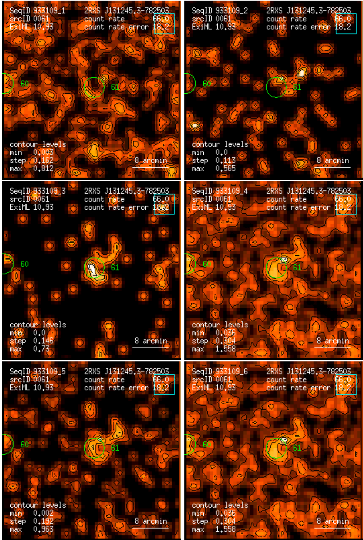
Figure 61: RASS 933109: detection 0061: band rate images, Gaussian filter: (1) PSPC channels 11 – 41, (2) 52 – 90, (3) 91 – 201, (4) 11 – 235, (5) 52 – 201, (6) 11 – 201. Broad band rates in counts/ks. Band rate contour levels in counts/ks/arcmin 2 .
