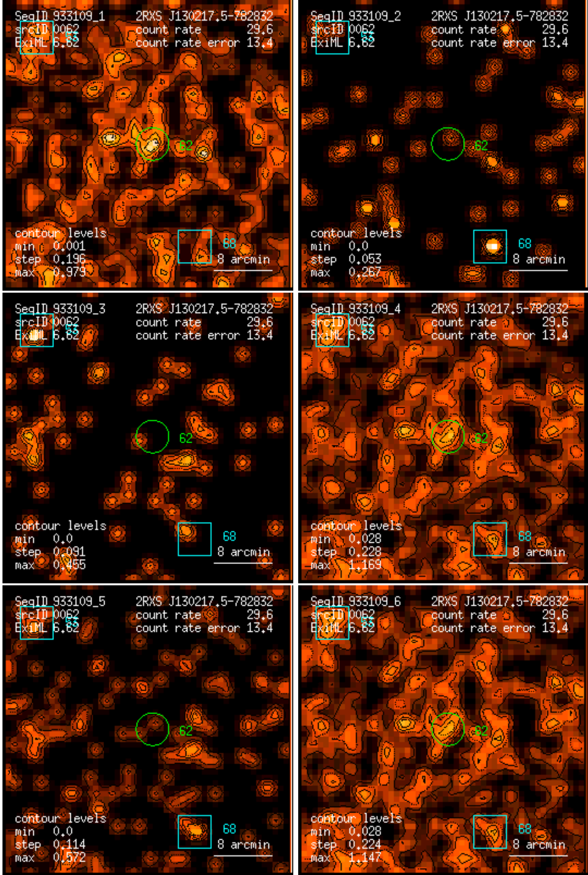
Figure 62: RASS 933109: detection 0062: band rate images, Gaussian filter: (1) PSPC channels 11 – 41, (2) 52 – 90, (3) 91 – 201, (4) 11 – 235, (5) 52 – 201, (6) 11 – 201. Broad band rates in counts/ks. Band rate contour levels in counts/ks/arcmin 2 .
