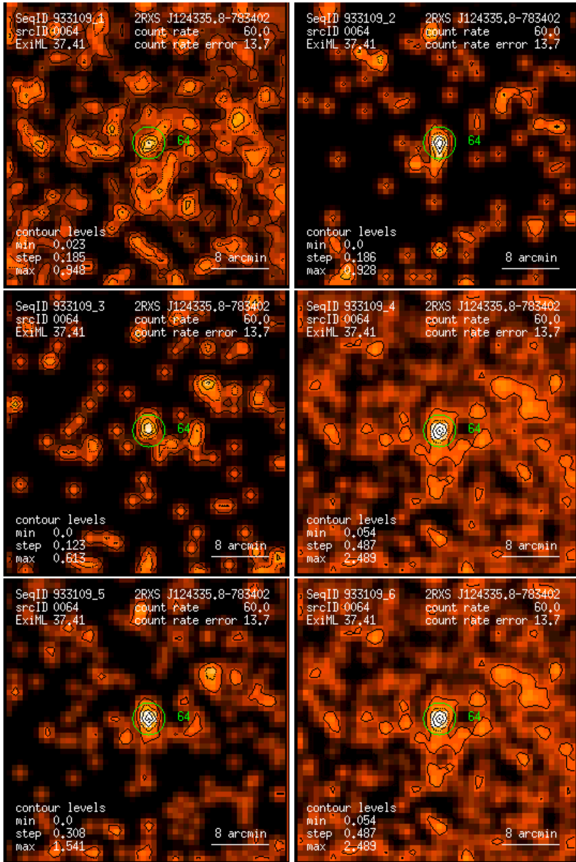
Figure 64: RASS 933109: detection 0064: band rate images, Gaussian filter: (1) PSPC channels 11 – 41, (2) 52 – 90, (3) 91 – 201, (4) 11 – 235, (5) 52 – 201, (6) 11 – 201. Broad band rates in counts/ks. Band rate contour levels in counts/ks/arcmin 2 .
