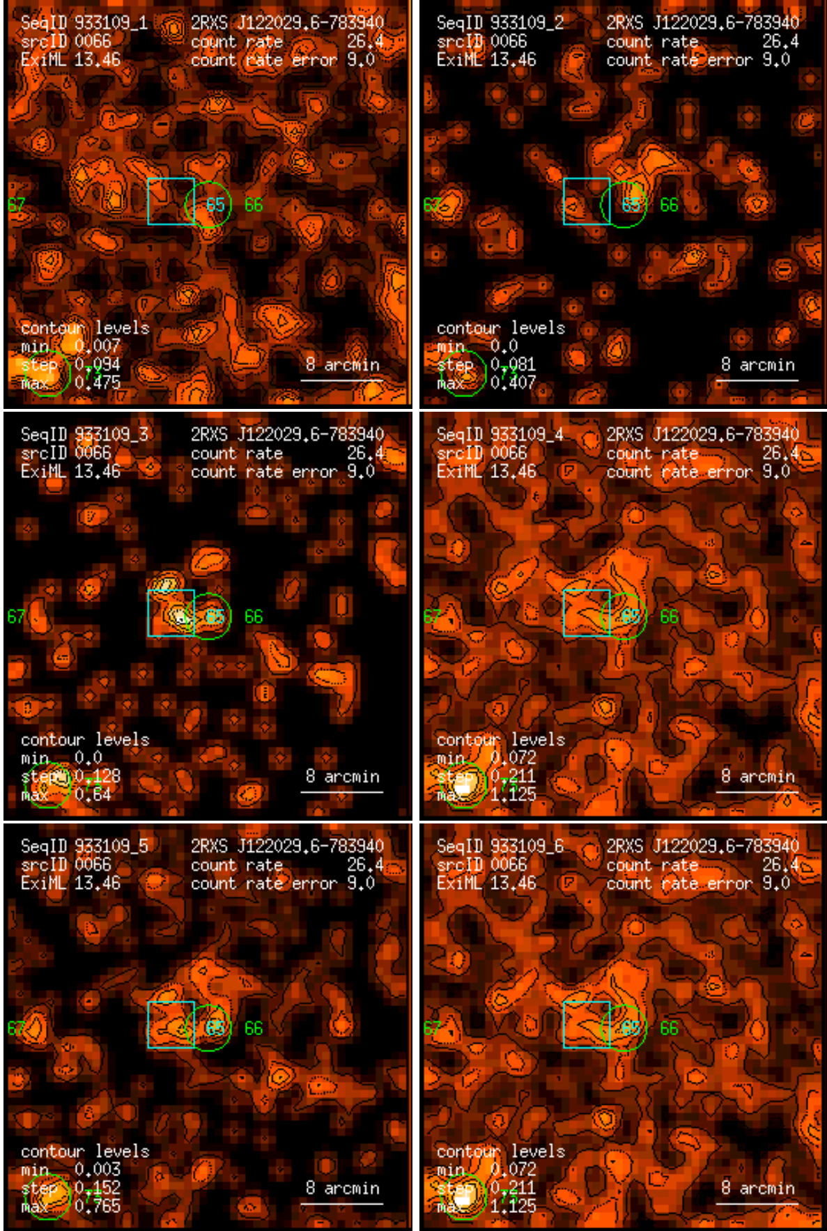
Figure 66: RASS 933109: detection 0066: band rate images, Gaussian filter: (1) PSPC channels 11 – 41, (2) 52 – 90, (3) 91 – 201, (4) 11 – 235, (5) 52 – 201, (6) 11 – 201. Broad band rates in counts/ks. Band rate contour levels in counts/ks/arcmin 2 .
