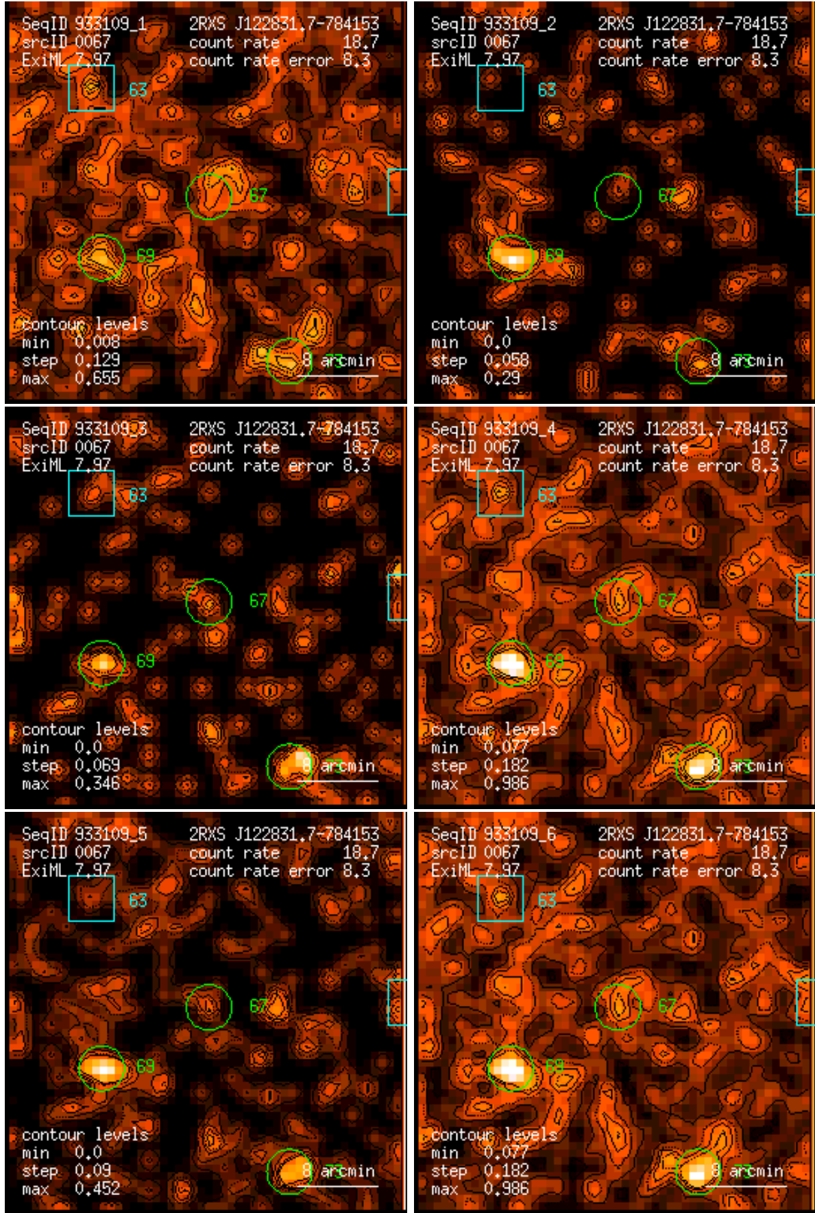
Figure 67: RASS 933109: detection 0067: band rate images, Gaussian filter: (1) PSPC channels 11 – 41, (2) 52 – 90, (3) 91 – 201, (4) 11 – 235, (5) 52 – 201, (6) 11 – 201. Broad band rates in counts/ks. Band rate contour levels in counts/ks/arcmin 2 .
