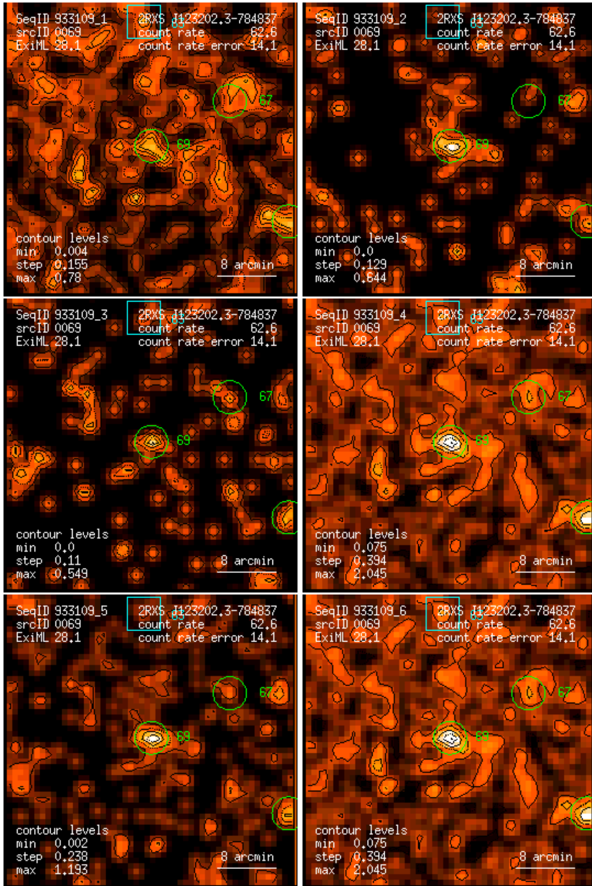
Figure 69: RASS 933109: detection 0069: band rate images, Gaussian filter: (1) PSPC channels 11 – 41, (2) 52 – 90, (3) 91 – 201, (4) 11 – 235, (5) 52 – 201, (6) 11 – 201. Broad band rates in counts/ks. Band rate contour levels in counts/ks/arcmin 2 .
