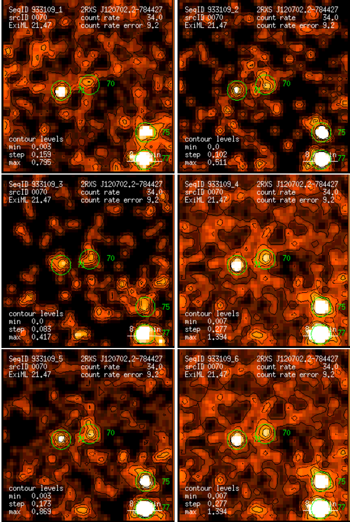
Figure 70: RASS 933109: detection 0070: band rate images, Gaussian filter: (1) PSPC channels 11 – 41, (2) 52 – 90, (3) 91 – 201, (4) 11 – 235, (5) 52 – 201, (6) 11 – 201. Broad band rates in counts/ks. Band rate contour levels in counts/ks/arcmin 2 .
