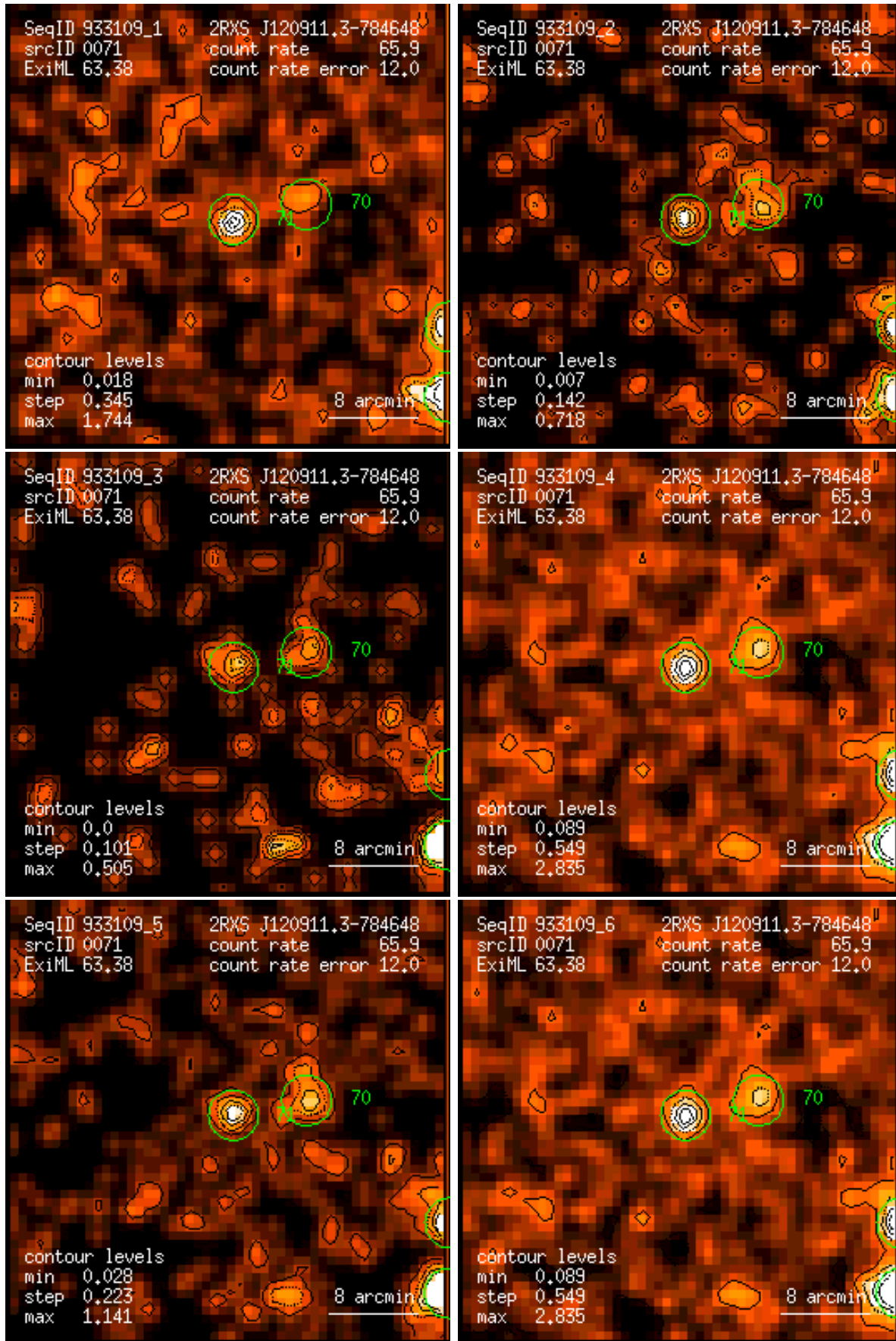
Figure 71: RASS 933109: detection 0071: band rate images, Gaussian filter: (1) PSPC channels 11 – 41, (2) 52 – 90, (3) 91 – 201, (4) 11 – 235, (5) 52 – 201, (6) 11 – 201. Broad band rates in counts/ks. Band rate contour levels in counts/ks/arcmin 2 .
