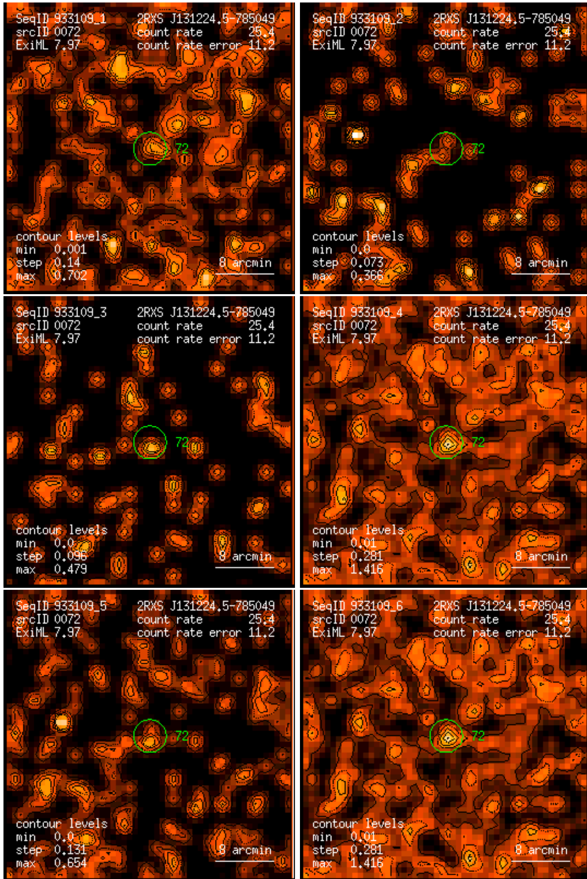
Figure 72: RASS 933109: detection 0072: band rate images, Gaussian filter: (1) PSPC channels 11 – 41, (2) 52 – 90, (3) 91 – 201, (4) 11 – 235, (5) 52 – 201, (6) 11 – 201. Broad band rates in counts/ks. Band rate contour levels in counts/ks/arcmin 2 .
