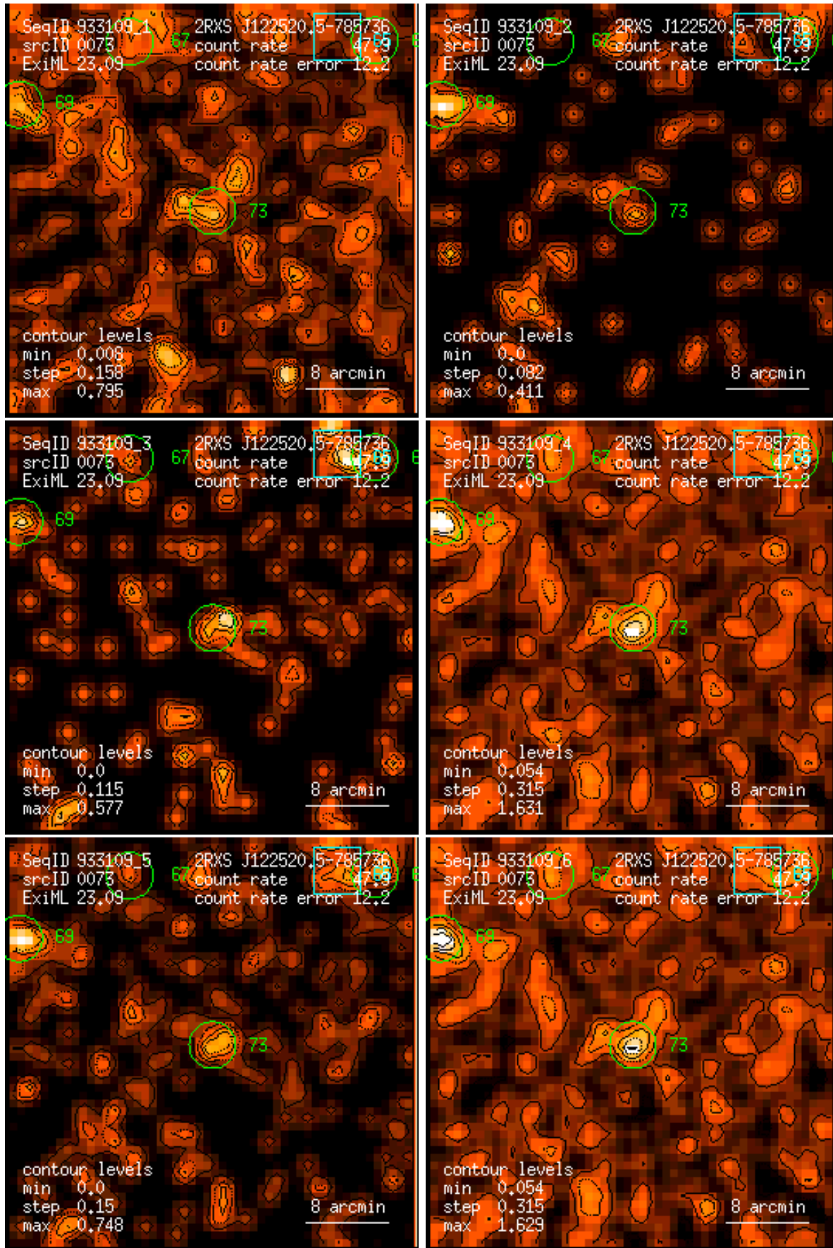
Figure 73: RASS 933109: detection 0073: band rate images, Gaussian filter: (1) PSPC channels 11 – 41, (2) 52 – 90, (3) 91 – 201, (4) 11 – 235, (5) 52 – 201, (6) 11 – 201. Broad band rates in counts/ks. Band rate contour levels in counts/ks/arcmin 2 .
