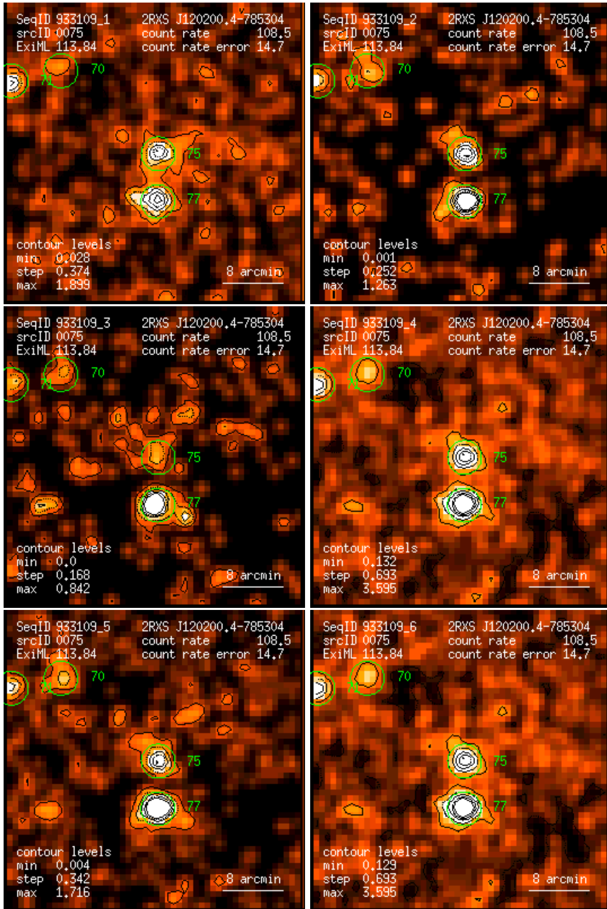
Figure 75: RASS 933109: detection 0075: band rate images, Gaussian filter: (1) PSPC channels 11 – 41, (2) 52 – 90, (3) 91 – 201, (4) 11 – 235, (5) 52 – 201, (6) 11 – 201. Broad band rates in counts/ks. Band rate contour levels in counts/ks/arcmin 2 .
