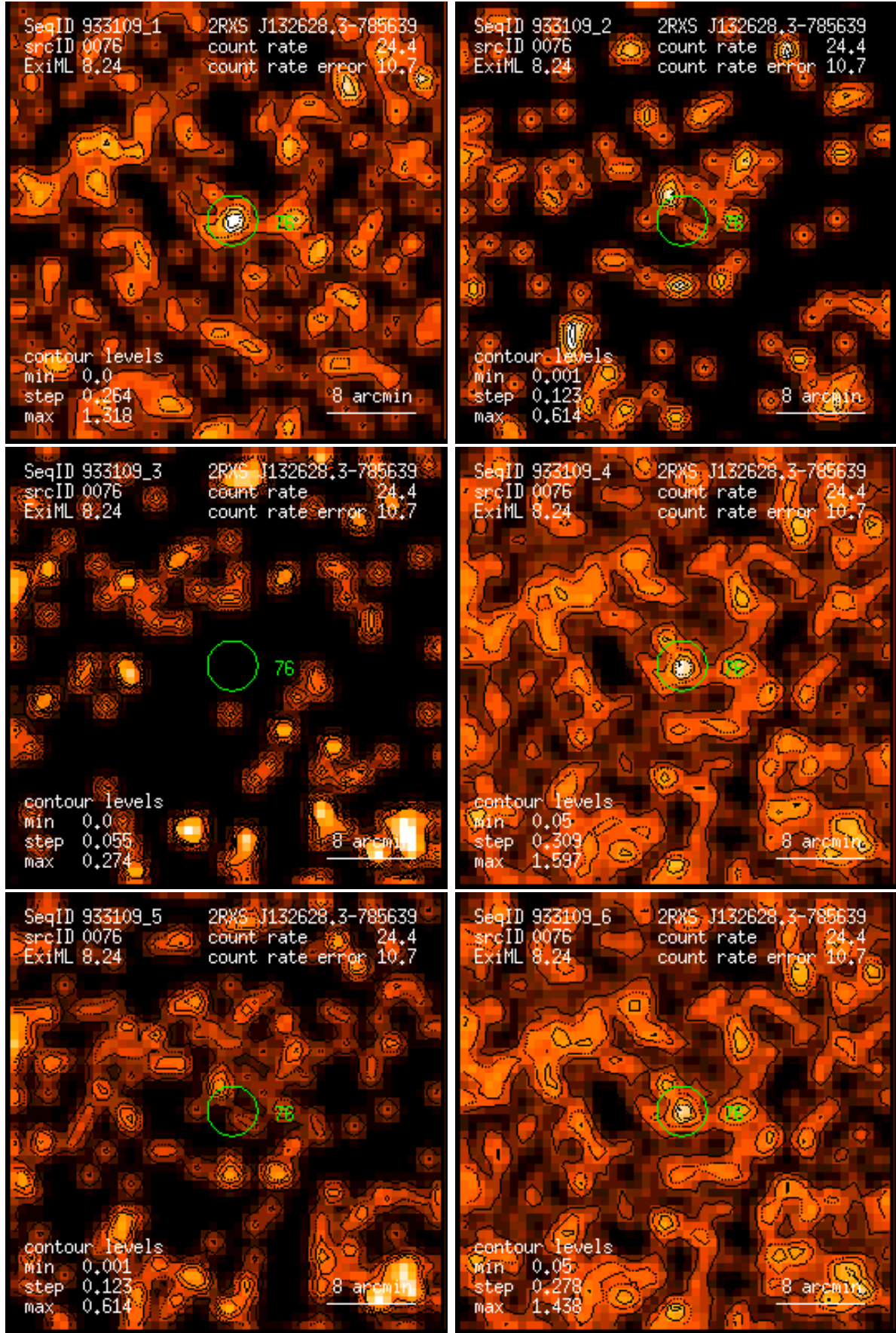
Figure 76: RASS 933109: detection 0076: band rate images, Gaussian filter: (1) PSPC channels 11 – 41, (2) 52 – 90, (3) 91 – 201, (4) 11 – 235, (5) 52 – 201, (6) 11 – 201. Broad band rates in counts/ks. Band rate contour levels in counts/ks/arcmin 2 .
