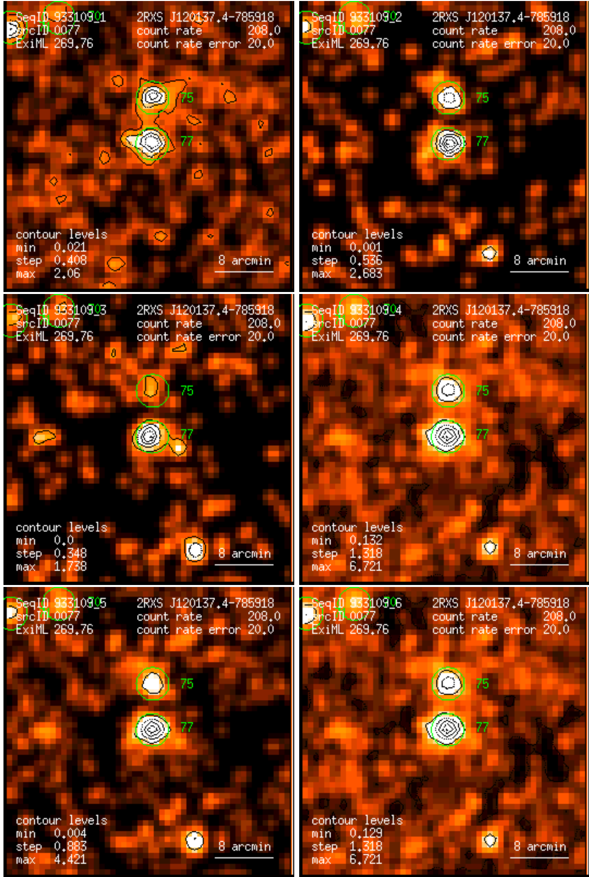
Figure 77: RASS 933109: detection 0077: band rate images, Gaussian filter: (1) PSPC channels 11 – 41, (2) 52 – 90, (3) 91 – 201, (4) 11 – 235, (5) 52 – 201, (6) 11 – 201. Broad band rates in counts/ks. Band rate contour levels in counts/ks/arcmin 2 .
