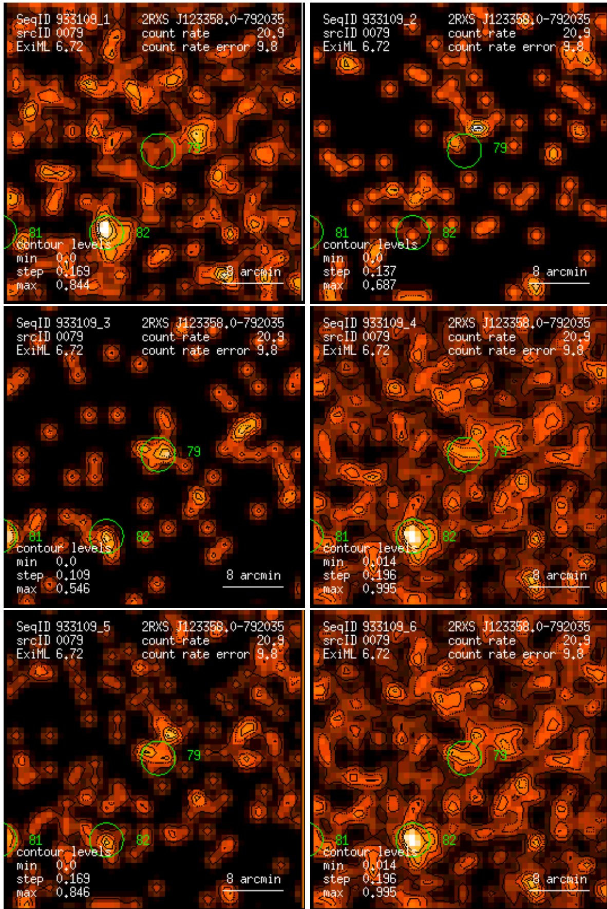
Figure 79: RASS 933109: detection 0079: band rate images, Gaussian filter: (1) PSPC channels 11 – 41, (2) 52 – 90, (3) 91 – 201, (4) 11 – 235, (5) 52 – 201, (6) 11 – 201. Broad band rates in counts/ks. Band rate contour levels in counts/ks/arcmin 2 .
