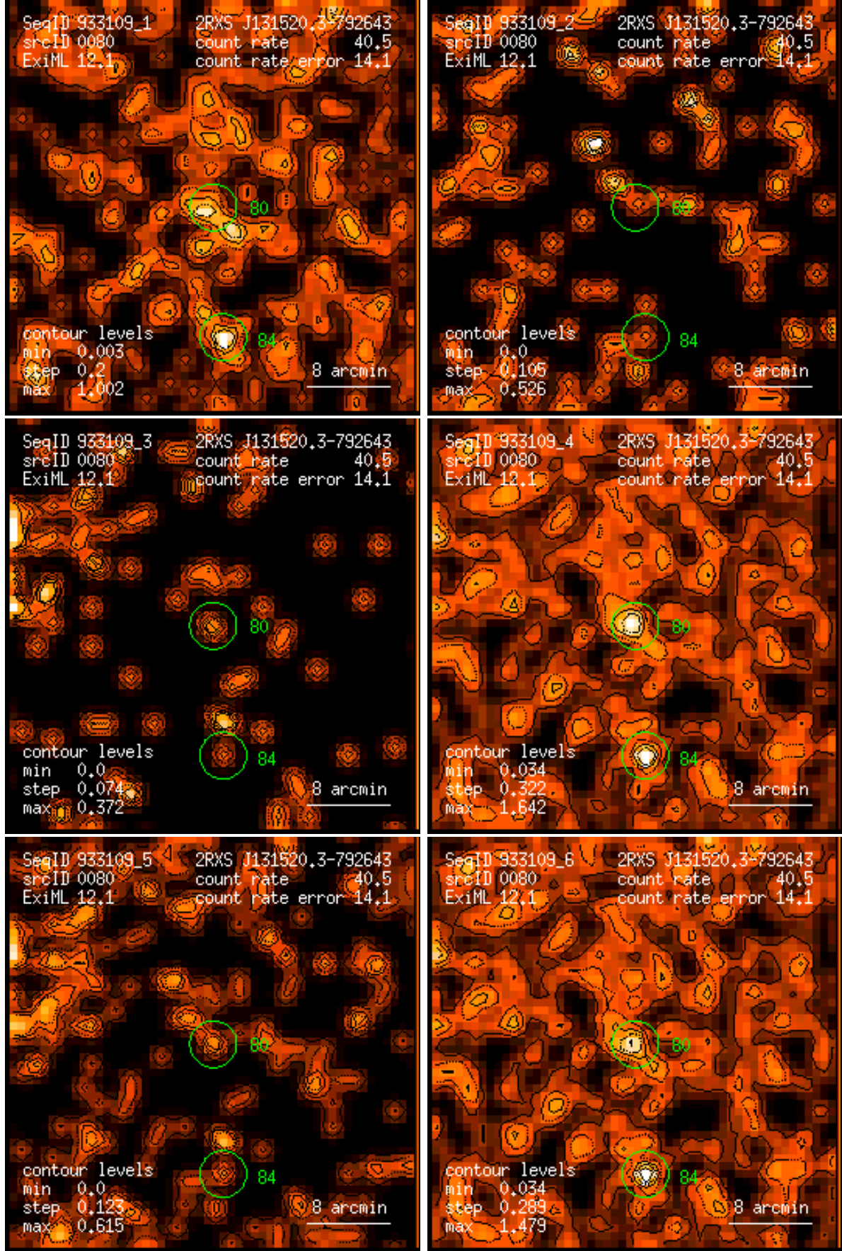
Figure 80: RASS 933109: detection 0080: band rate images, Gaussian filter: (1) PSPC channels 11 – 41, (2) 52 – 90, (3) 91 – 201, (4) 11 – 235, (5) 52 – 201, (6) 11 – 201. Broad band rates in counts/ks. Band rate contour levels in counts/ks/arcmin 2 .
