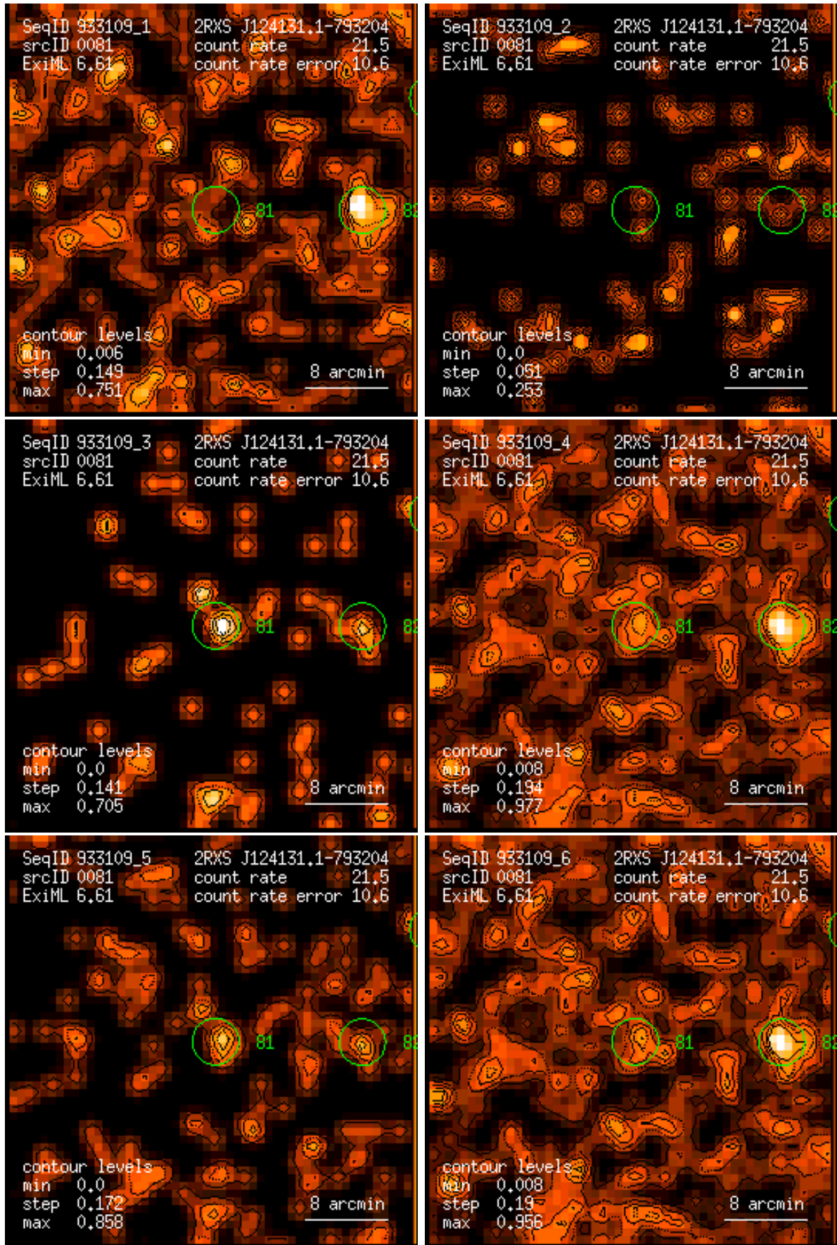
Figure 81: RASS 933109: detection 0081: band rate images, Gaussian filter: (1) PSPC channels 11 – 41, (2) 52 – 90, (3) 91 – 201, (4) 11 – 235, (5) 52 – 201, (6) 11 – 201. Broad band rates in counts/ks. Band rate contour levels in counts/ks/arcmin 2 .
