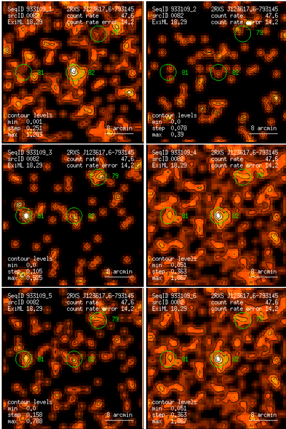
Figure 82: RASS 933109: detection 0082: band rate images, Gaussian filter: (1) PSPC channels 11 – 41, (2) 52 – 90, (3) 91 – 201, (4) 11 – 235, (5) 52 – 201, (6) 11 – 201. Broad band rates in counts/ks. Band rate contour levels in counts/ks/arcmin 2 .
