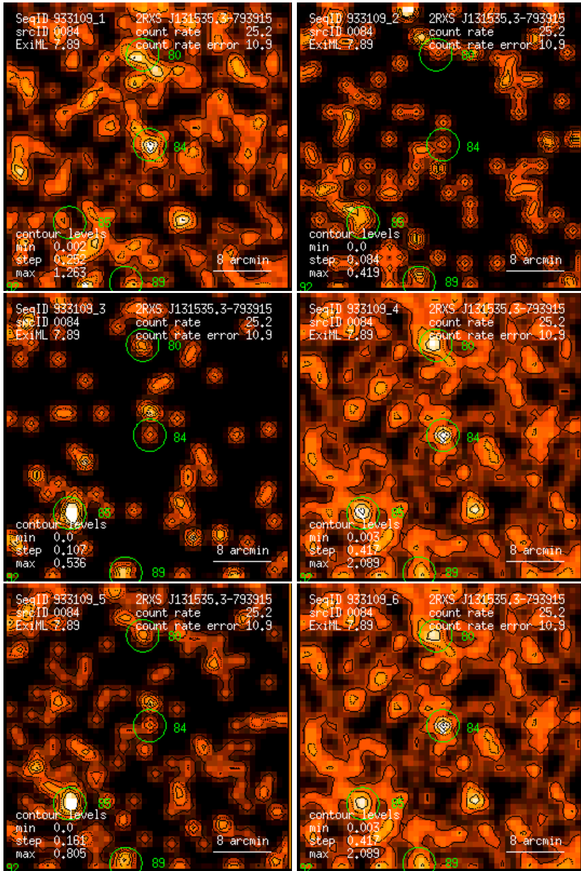
Figure 84: RASS 933109: detection 0084: band rate images, Gaussian filter: (1) PSPC channels 11 – 41, (2) 52 – 90, (3) 91 – 201, (4) 11 – 235, (5) 52 – 201, (6) 11 – 201. Broad band rates in counts/ks. Band rate contour levels in counts/ks/arcmin 2 .
