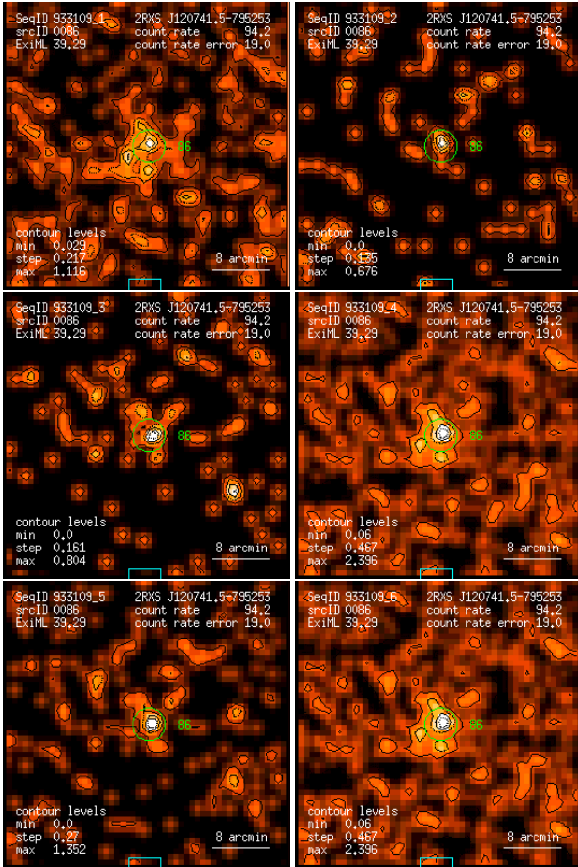
Figure 86: RASS 933109: detection 0086: band rate images, Gaussian filter: (1) PSPC channels 11 – 41, (2) 52 – 90, (3) 91 – 201, (4) 11 – 235, (5) 52 – 201, (6) 11 – 201. Broad band rates in counts/ks. Band rate contour levels in counts/ks/arcmin 2 .
