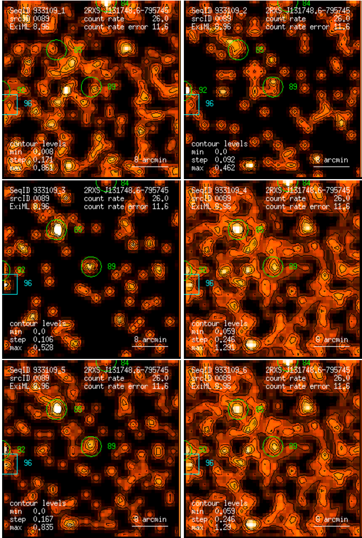
Figure 89: RASS 933109: detection 0089: band rate images, Gaussian filter: (1) PSPC channels 11 – 41, (2) 52 – 90, (3) 91 – 201, (4) 11 – 235, (5) 52 – 201, (6) 11 – 201. Broad band rates in counts/ks. Band rate contour levels in counts/ks/arcmin 2 .
