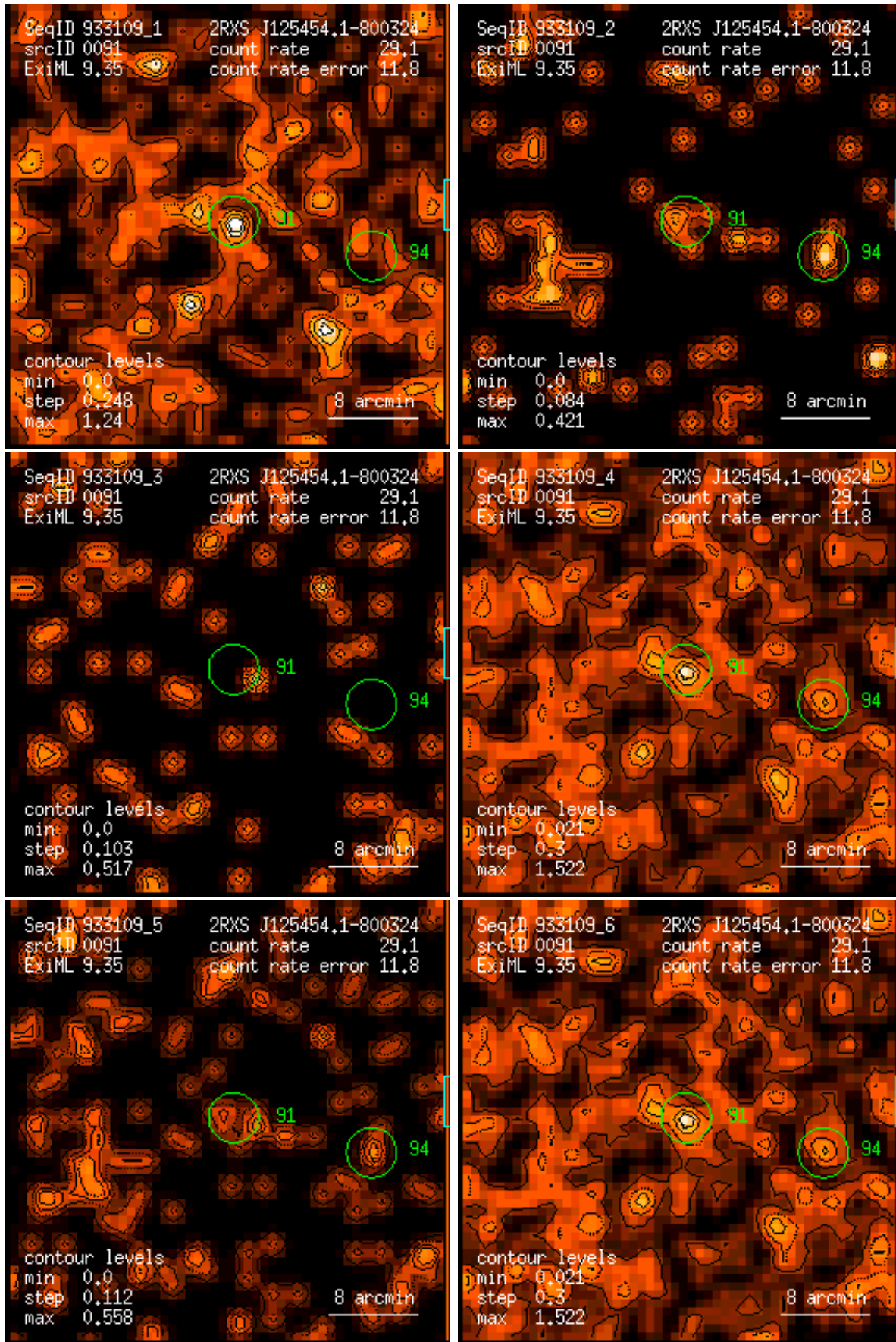
Figure 91: RASS 933109: detection 0091: band rate images, Gaussian filter: (1) PSPC channels 11 – 41, (2) 52 – 90, (3) 91 – 201, (4) 11 – 235, (5) 52 – 201, (6) 11 – 201. Broad band rates in counts/ks. Band rate contour levels in counts/ks/arcmin 2 .
