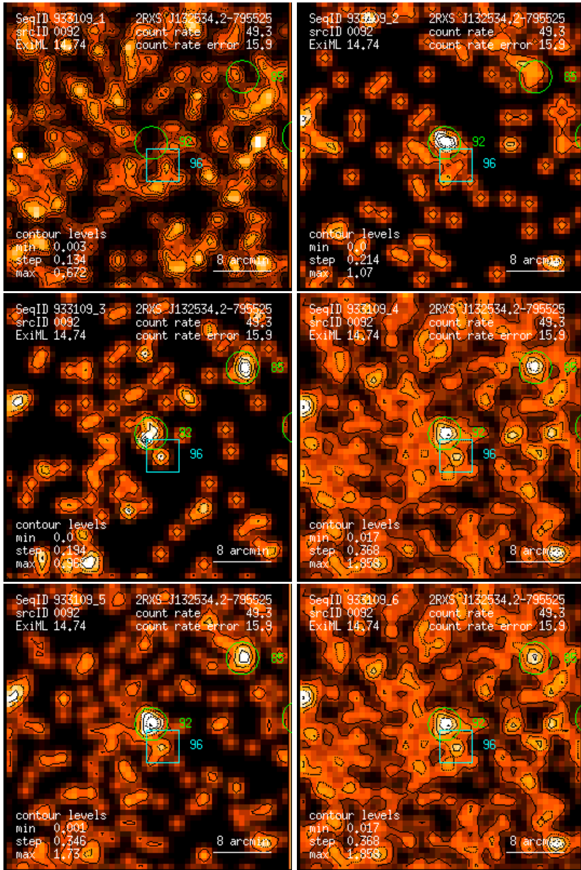
Figure 92: RASS 933109: detection 0092: band rate images, Gaussian filter: (1) PSPC channels 11 – 41, (2) 52 – 90, (3) 91 – 201, (4) 11 – 235, (5) 52 – 201, (6) 11 – 201. Broad band rates in counts/ks. Band rate contour levels in counts/ks/arcmin 2 .
