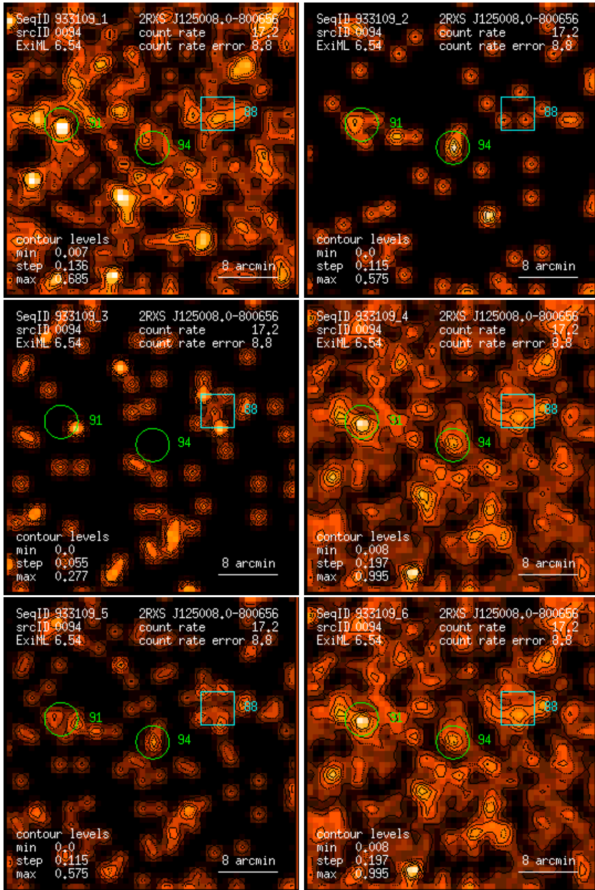
Figure 94: RASS 933109: detection 0094: band rate images, Gaussian filter: (1) PSPC channels 11 – 41, (2) 52 – 90, (3) 91 – 201, (4) 11 – 235, (5) 52 – 201, (6) 11 – 201. Broad band rates in counts/ks. Band rate contour levels in counts/ks/arcmin 2 .
