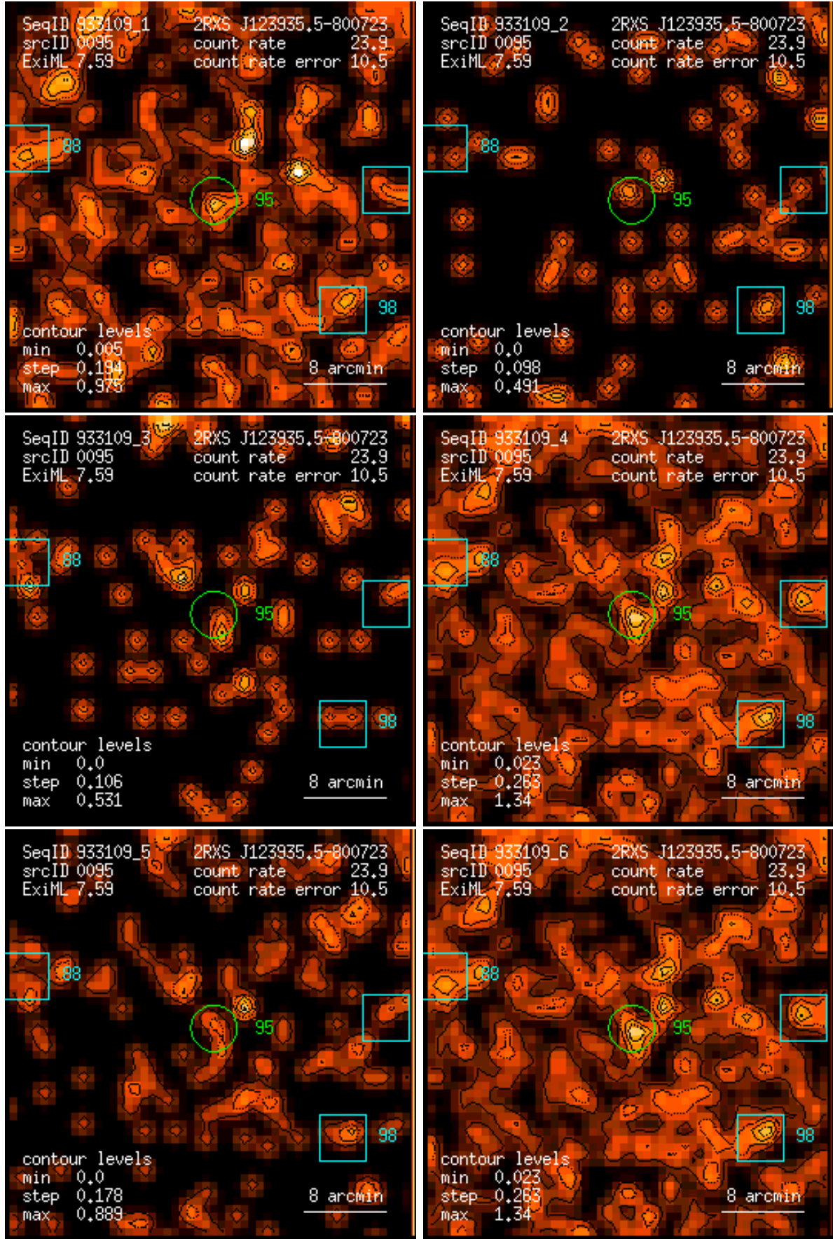
Figure 95: RASS 933109: detection 0095: band rate images, Gaussian filter: (1) PSPC channels 11 – 41, (2) 52 – 90, (3) 91 – 201, (4) 11 – 235, (5) 52 – 201, (6) 11 – 201. Broad band rates in counts/ks. Band rate contour levels in counts/ks/arcmin 2 .
