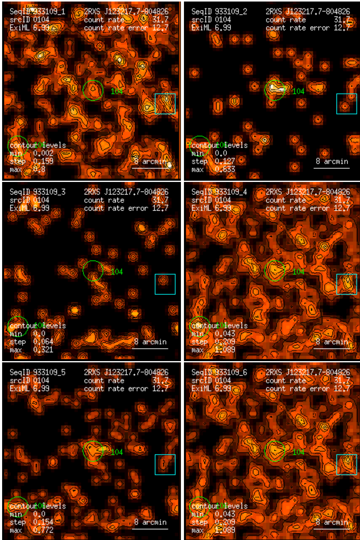
Figure 104: RASS 933109: detection 0104: band rate images, Gaussian filter: (1) PSPC channels 11 – 41, (2) 52 – 90, (3) 91 – 201, (4) 11 – 235, (5) 52 – 201, (6) 11 – 201. Broad band rates in counts/ks. Band rate contour levels in counts/ks/arcmin 2 .
