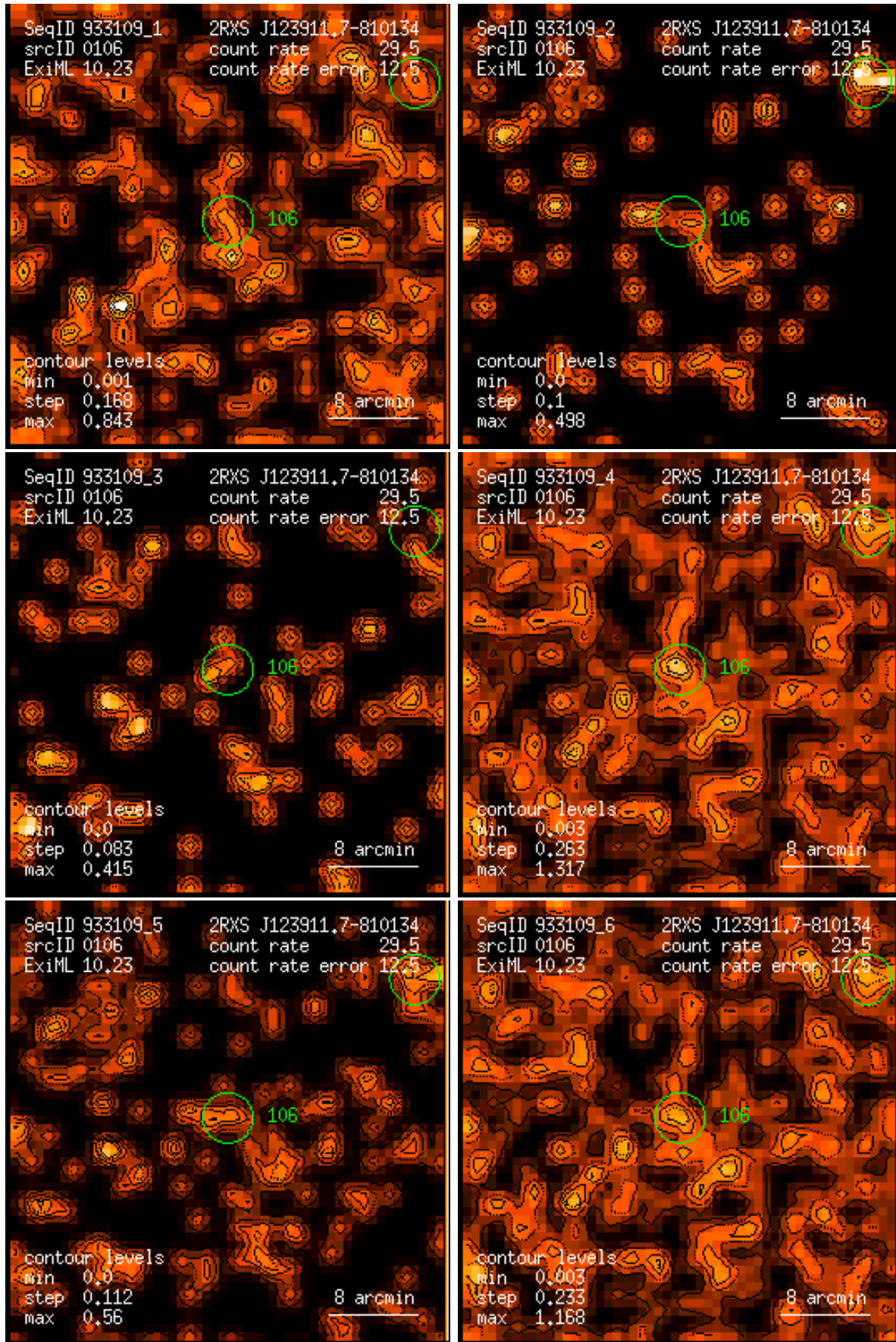
Figure 106: RASS 933109: detection 0106: band rate images, Gaussian filter: (1) PSPC channels 11 – 41, (2) 52 – 90, (3) 91 – 201, (4) 11 – 235, (5) 52 – 201, (6) 11 – 201. Broad band rates in counts/ks. Band rate contour levels in counts/ks/arcmin 2 .
