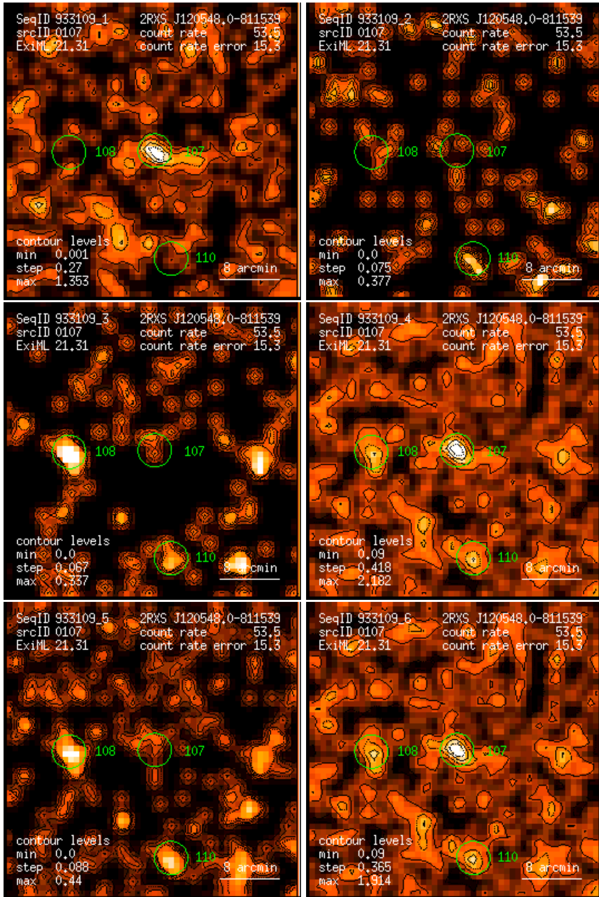
Figure 107: RASS 933109: detection 0107: band rate images, Gaussian filter: (1) PSPC channels 11 – 41, (2) 52 – 90, (3) 91 – 201, (4) 11 – 235, (5) 52 – 201, (6) 11 – 201. Broad band rates in counts/ks. Band rate contour levels in counts/ks/arcmin 2 .
