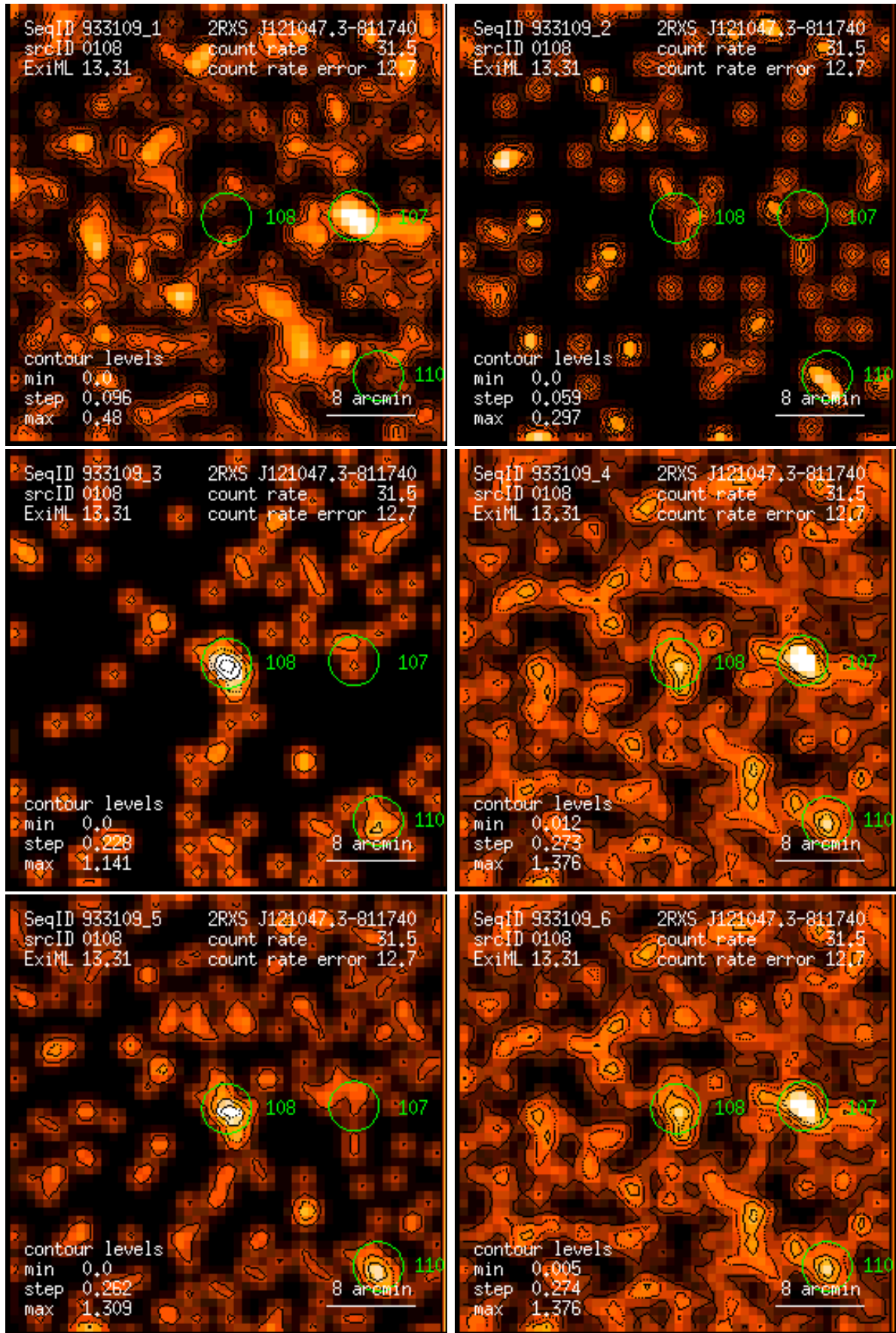
Figure 108: RASS 933109: detection 0108: band rate images, Gaussian filter: (1) PSPC channels 11 – 41, (2) 52 – 90, (3) 91 – 201, (4) 11 – 235, (5) 52 – 201, (6) 11 – 201. Broad band rates in counts/ks. Band rate contour levels in counts/ks/arcmin 2 .
