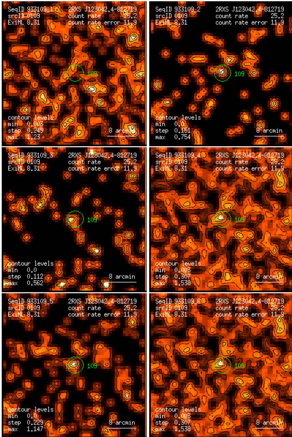
Figure 109: RASS 933109: detection 0109: band rate images, Gaussian filter: (1) PSPC channels 11 – 41, (2) 52 – 90, (3) 91 – 201, (4) 11 – 235, (5) 52 – 201, (6) 11 – 201. Broad band rates in counts/ks. Band rate contour levels in counts/ks/arcmin 2 .
