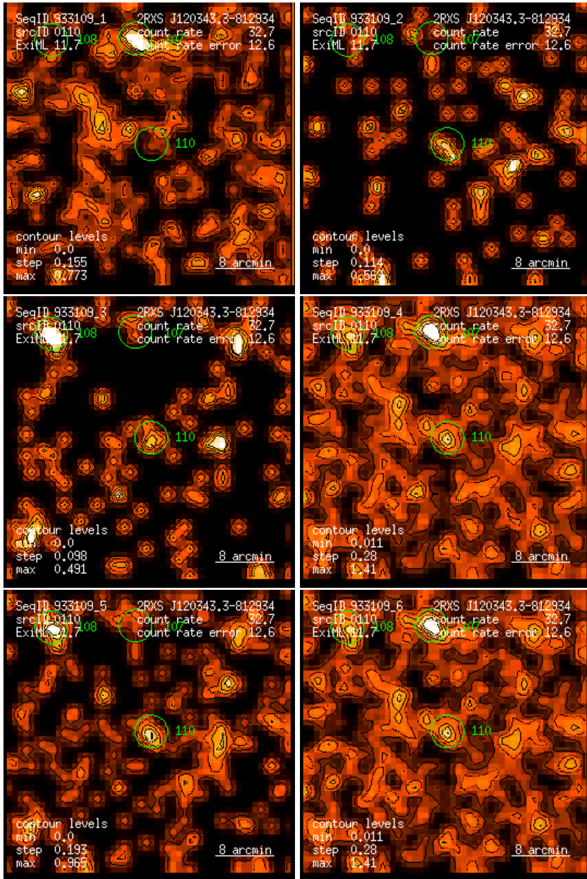
Figure 110: RASS 933109: detection 0110: band rate images, Gaussian filter: (1) PSPC channels 11 – 41, (2) 52 – 90, (3) 91 – 201, (4) 11 – 235, (5) 52 – 201, (6) 11 – 201. Broad band rates in counts/ks. Band rate contour levels in counts/ks/arcmin 2 .
