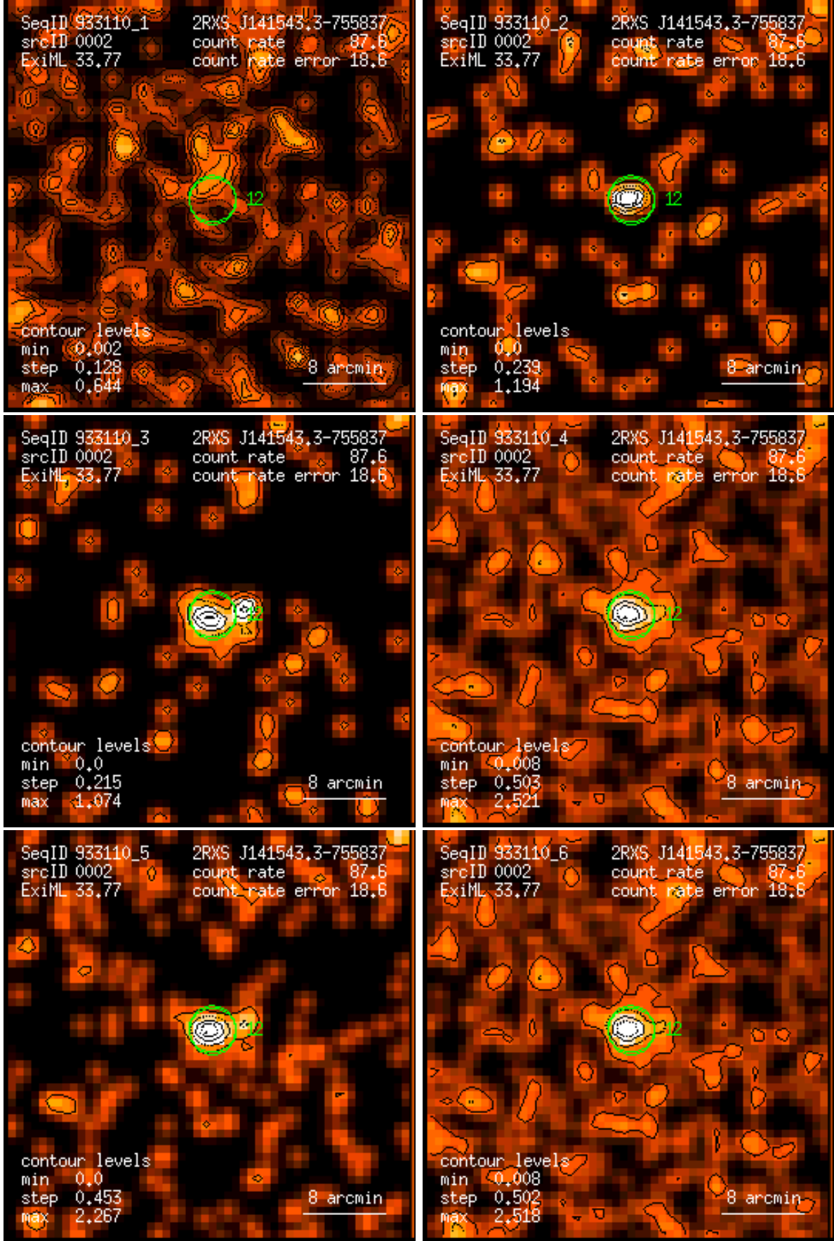
Figure 2: RASS 933110: detection 0002: band rate images, Gaussian filter: (1) PSPC channels 11 – 41, (2) 52 – 90, (3) 91 – 201, (4) 11 – 235, (5) 52 – 201, (6) 11 – 201. Broad band rates in counts/ks. Band rate contour levels in counts/ks/arcmin 2 .
