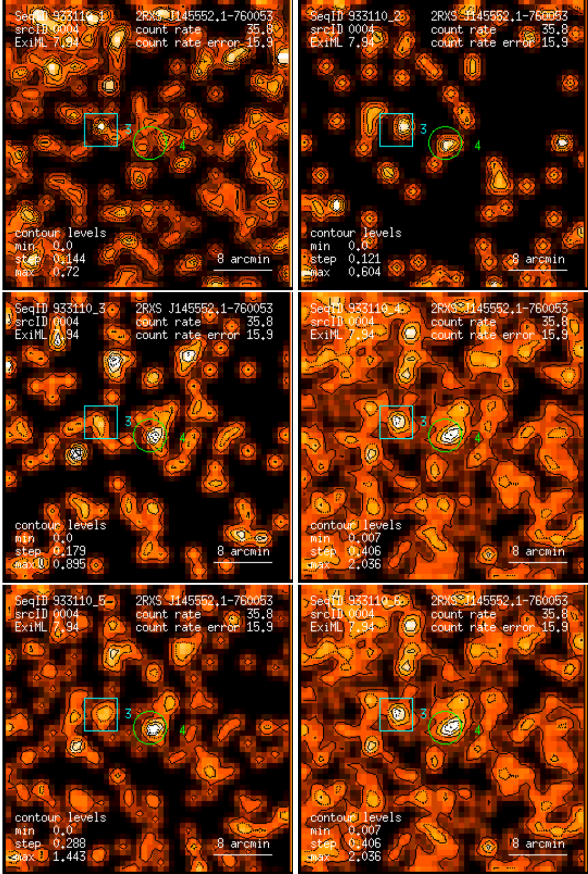
Figure 4: RASS 933110: detection 0004: band rate images, Gaussian filter: (1) PSPC channels 11 – 41, (2) 52 – 90, (3) 91 – 201, (4) 11 – 235, (5) 52 – 201, (6) 11 – 201. Broad band rates in counts/ks. Band rate contour levels in counts/ks/arcmin 2 .
