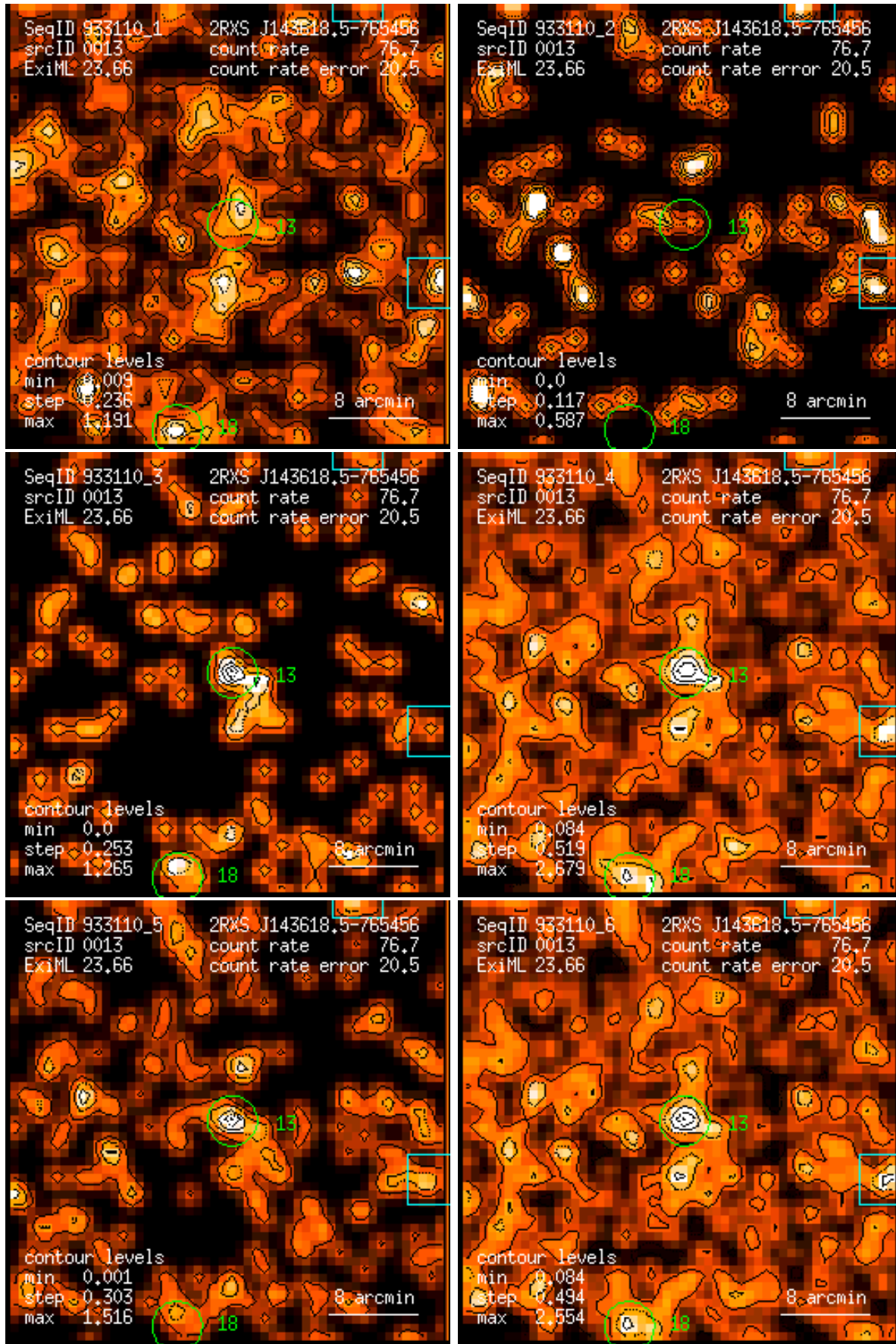
Figure 13: RASS 933110: detection 0013: band rate images, Gaussian filter: (1) PSPC channels 11 – 41, (2) 52 – 90, (3) 91 – 201, (4) 11 – 235, (5) 52 – 201, (6) 11 – 201. Broad band rates in counts/ks. Band rate contour levels in counts/ks/arcmin 2 .
