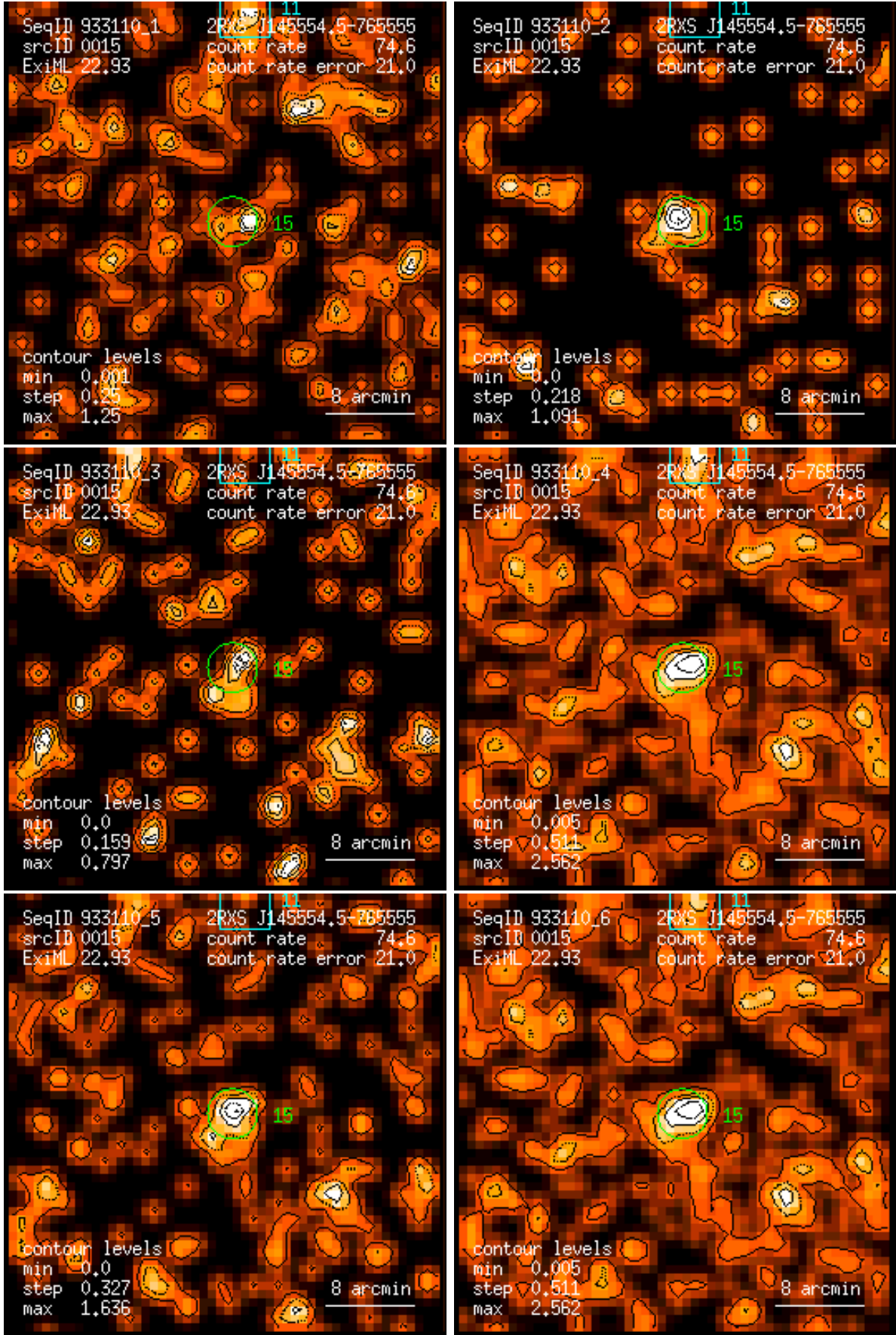
Figure 15: RASS 933110: detection 0015: band rate images, Gaussian filter: (1) PSPC channels 11 – 41, (2) 52 – 90, (3) 91 – 201, (4) 11 – 235, (5) 52 – 201, (6) 11 – 201. Broad band rates in counts/ks. Band rate contour levels in counts/ks/arcmin 2 .
