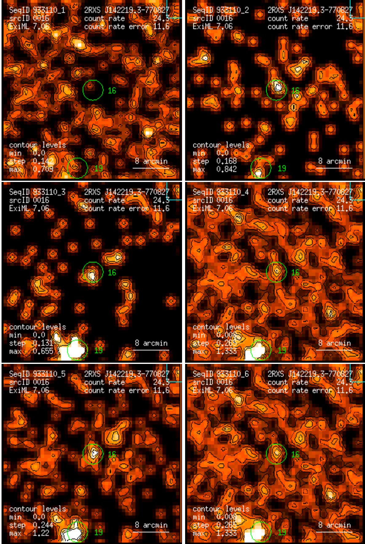
Figure 16: RASS 933110: detection 0016: band rate images, Gaussian filter: (1) PSPC channels 11 – 41, (2) 52 – 90, (3) 91 – 201, (4) 11 – 235, (5) 52 – 201, (6) 11 – 201. Broad band rates in counts/ks. Band rate contour levels in counts/ks/arcmin 2 .
