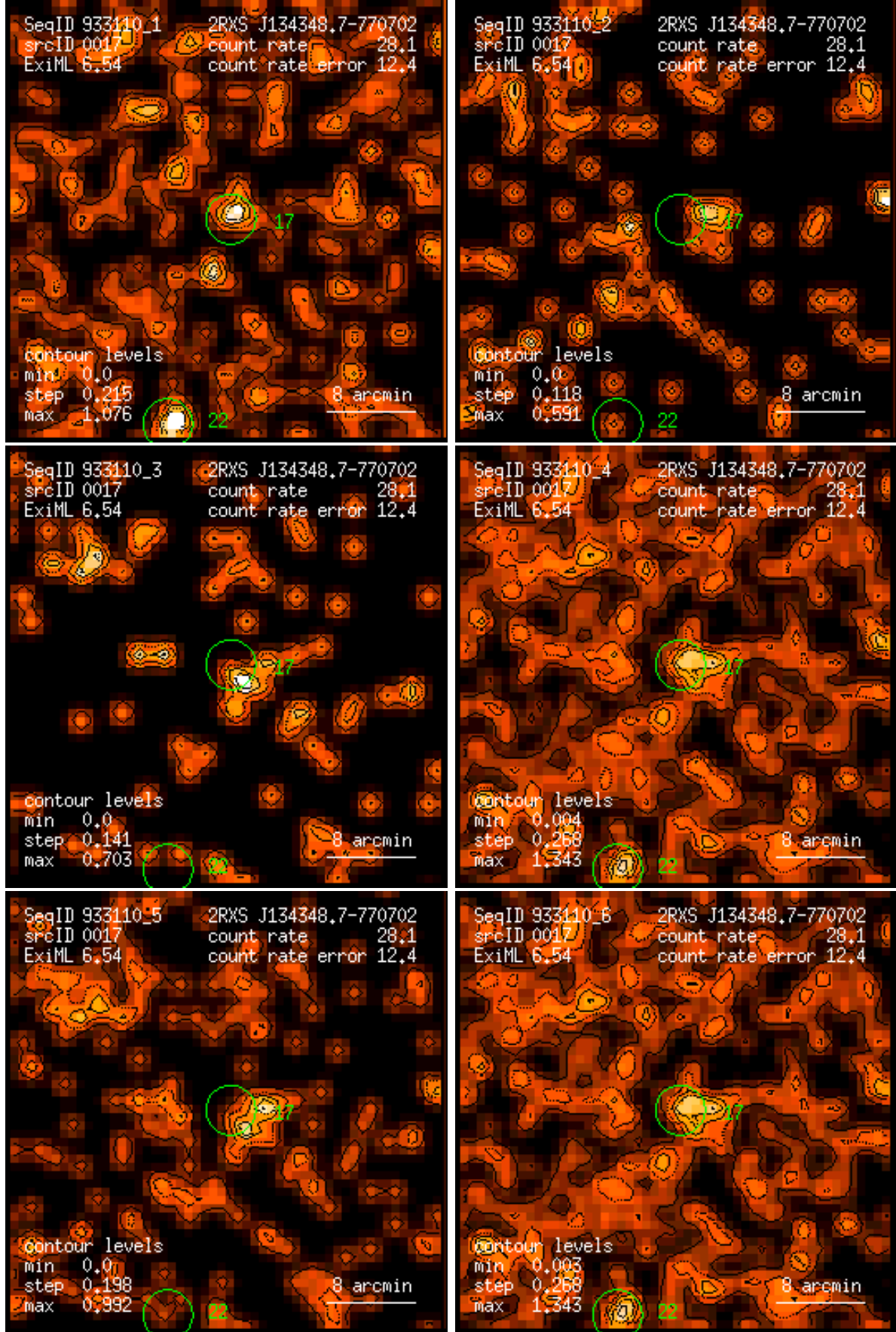
Figure 17: RASS 933110: detection 0017: band rate images, Gaussian filter: (1) PSPC channels 11 – 41, (2) 52 – 90, (3) 91 – 201, (4) 11 – 235, (5) 52 – 201, (6) 11 – 201. Broad band rates in counts/ks. Band rate contour levels in counts/ks/arcmin 2 .
