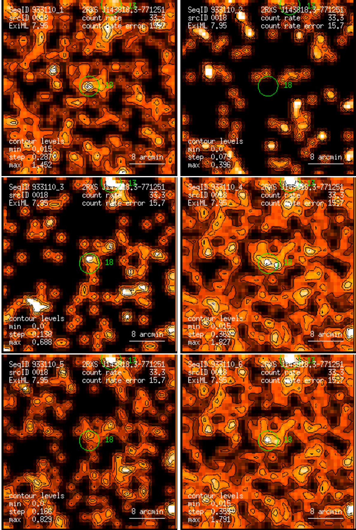
Figure 18: RASS 933110: detection 0018: band rate images, Gaussian filter: (1) PSPC channels 11 – 41, (2) 52 – 90, (3) 91 – 201, (4) 11 – 235, (5) 52 – 201, (6) 11 – 201. Broad band rates in counts/ks. Band rate contour levels in counts/ks/arcmin 2 .
