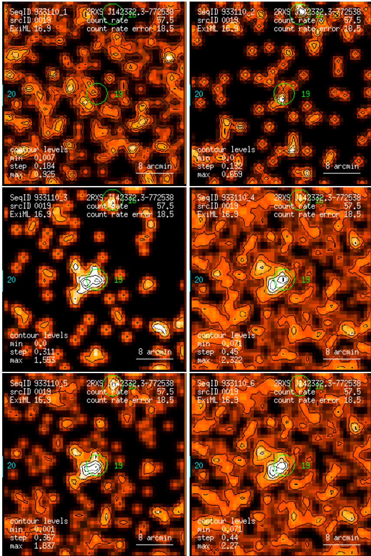
Figure 19: RASS 933110: detection 0019: band rate images, Gaussian filter: (1) PSPC channels 11 – 41, (2) 52 – 90, (3) 91 – 201, (4) 11 – 235, (5) 52 – 201, (6) 11 – 201. Broad band rates in counts/ks. Band rate contour levels in counts/ks/arcmin 2 .
