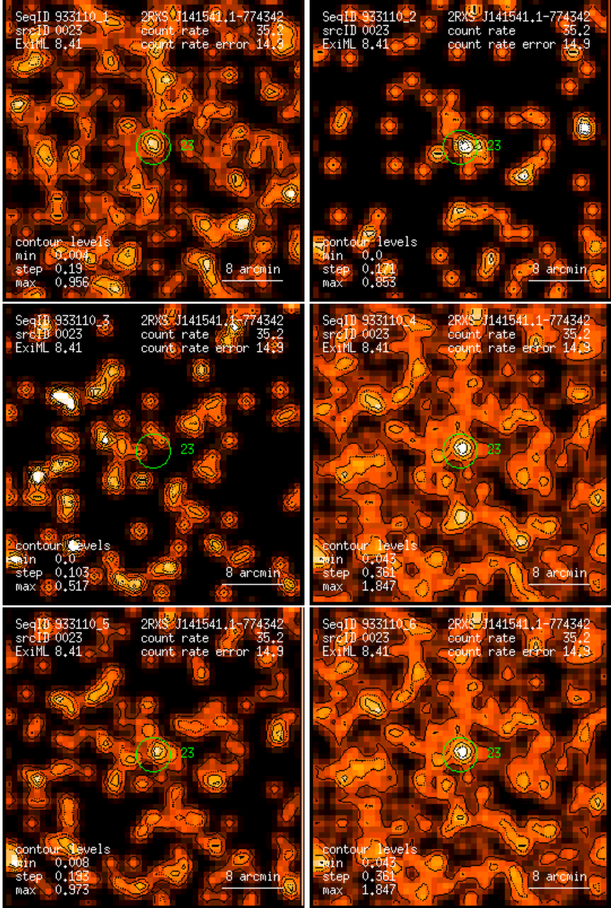
Figure 23: RASS 933110: detection 0023: band rate images, Gaussian filter: (1) PSPC channels 11 – 41, (2) 52 – 90, (3) 91 – 201, (4) 11 – 235, (5) 52 – 201, (6) 11 – 201. Broad band rates in counts/ks. Band rate contour levels in counts/ks/arcmin 2 .
