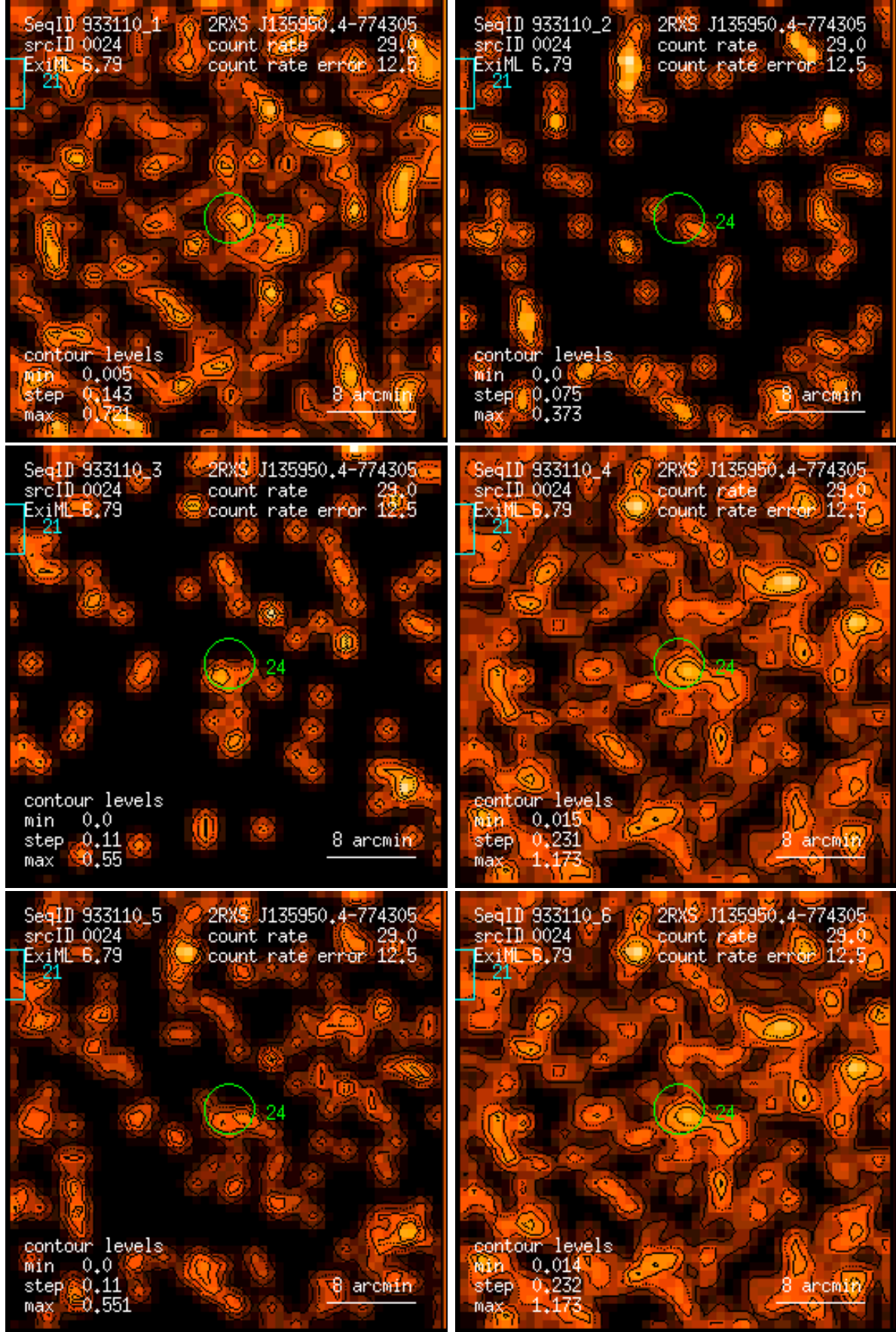
Figure 24: RASS 933110: detection 0024: band rate images, Gaussian filter: (1) PSPC channels 11 – 41, (2) 52 – 90, (3) 91 – 201, (4) 11 – 235, (5) 52 – 201, (6) 11 – 201. Broad band rates in counts/ks. Band rate contour levels in counts/ks/arcmin 2 .
