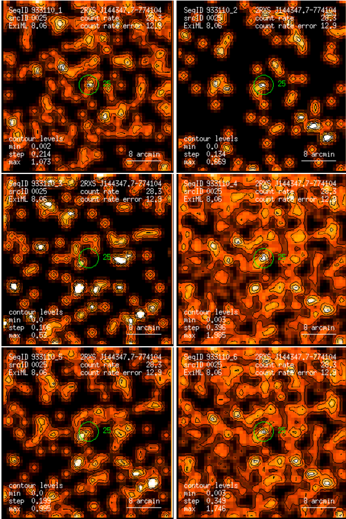
Figure 25: RASS 933110: detection 0025: band rate images, Gaussian filter: (1) PSPC channels 11 – 41, (2) 52 – 90, (3) 91 – 201, (4) 11 – 235, (5) 52 – 201, (6) 11 – 201. Broad band rates in counts/ks. Band rate contour levels in counts/ks/arcmin 2 .
