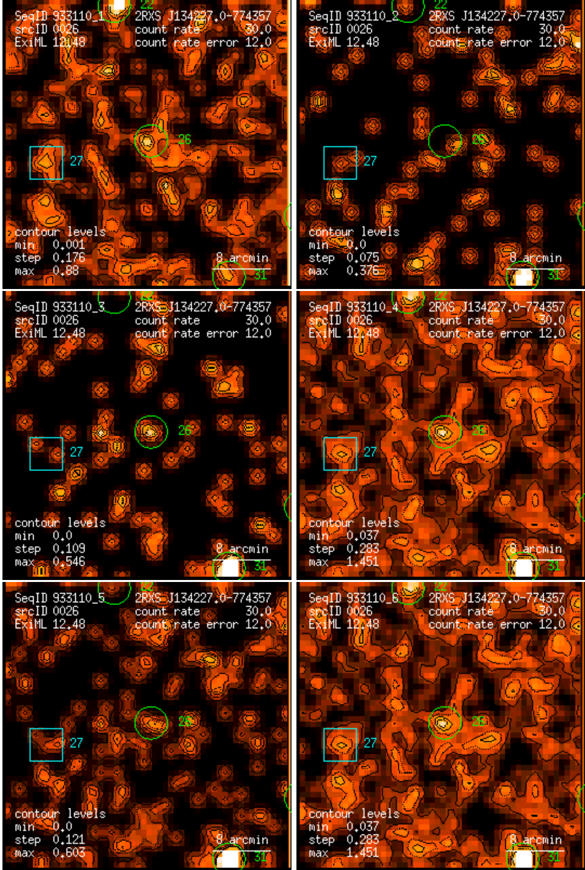
Figure 26: RASS 933110: detection 0026: band rate images, Gaussian filter: (1) PSPC channels 11 – 41, (2) 52 – 90, (3) 91 – 201, (4) 11 – 235, (5) 52 – 201, (6) 11 – 201. Broad band rates in counts/ks. Band rate contour levels in counts/ks/arcmin 2 .
