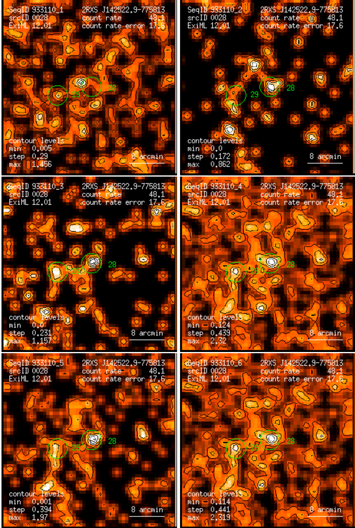
Figure 28: RASS 933110: detection 0028: band rate images, Gaussian filter: (1) PSPC channels 11 – 41, (2) 52 – 90, (3) 91 – 201, (4) 11 – 235, (5) 52 – 201, (6) 11 – 201. Broad band rates in counts/ks. Band rate contour levels in counts/ks/arcmin 2 .
