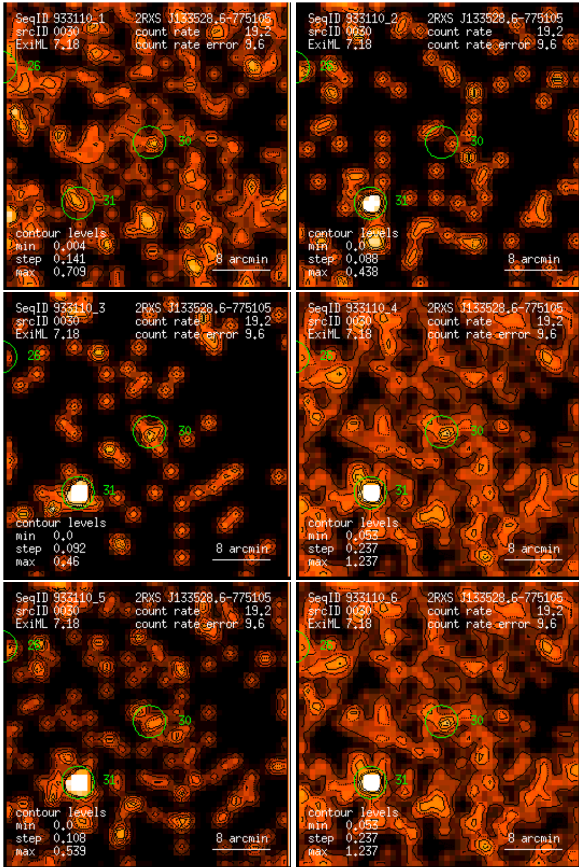
Figure 30: RASS 933110: detection 0030: band rate images, Gaussian filter: (1) PSPC channels 11 – 41, (2) 52 – 90, (3) 91 – 201, (4) 11 – 235, (5) 52 – 201, (6) 11 – 201. Broad band rates in counts/ks. Band rate contour levels in counts/ks/arcmin 2 .
