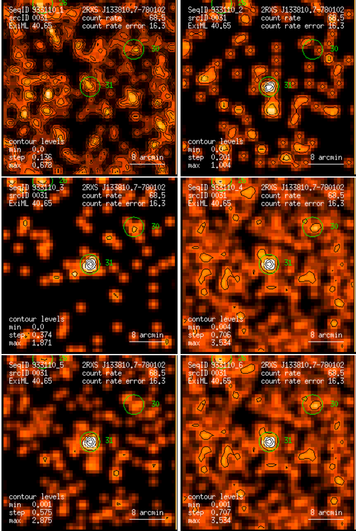
Figure 31: RASS 933110: detection 0031: band rate images, Gaussian filter: (1) PSPC channels 11 – 41, (2) 52 – 90, (3) 91 – 201, (4) 11 – 235, (5) 52 – 201, (6) 11 – 201. Broad band rates in counts/ks. Band rate contour levels in counts/ks/arcmin 2 .
