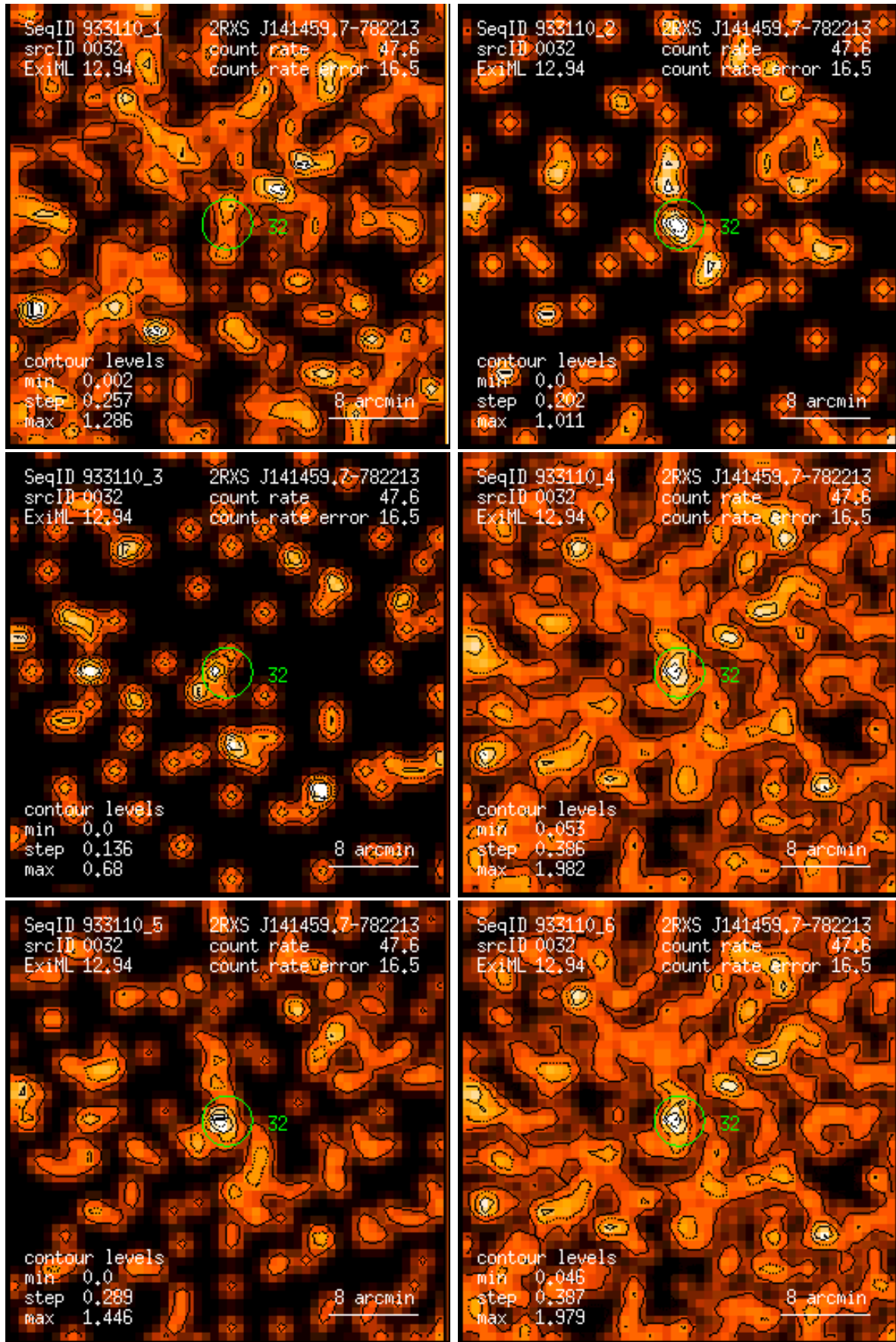
Figure 32: RASS 933110: detection 0032: band rate images, Gaussian filter: (1) PSPC channels 11 – 41, (2) 52 – 90, (3) 91 – 201, (4) 11 – 235, (5) 52 – 201, (6) 11 – 201. Broad band rates in counts/ks. Band rate contour levels in counts/ks/arcmin 2 .
